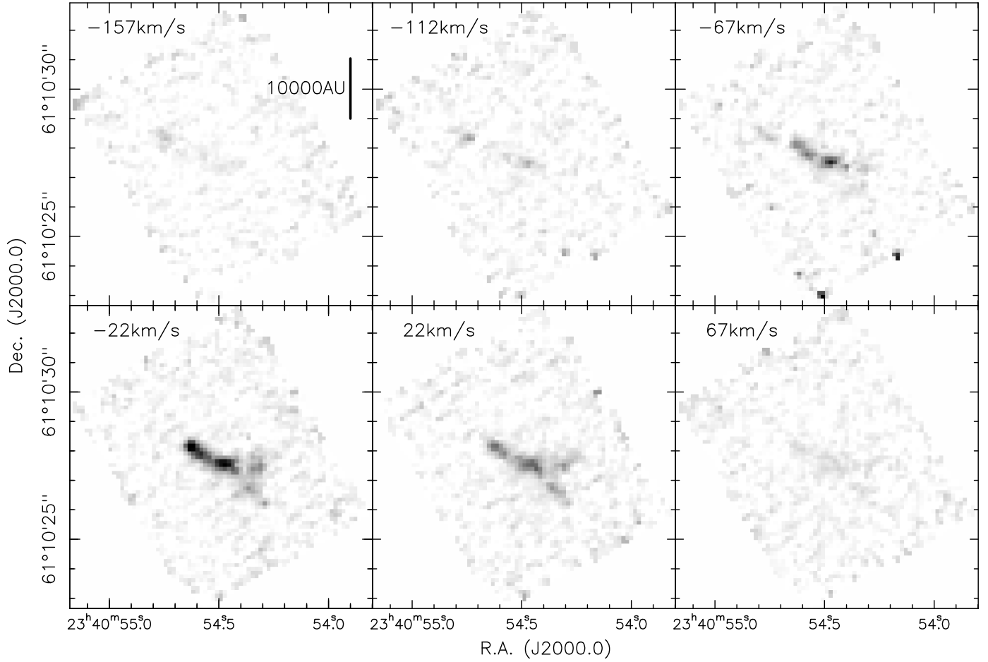
Fig. 7. Channel map of the \text{FeII}[(^4\text{F}_{9/2} - ^6\text{D}_{9/2})] line at 5.34 \mu\text{m} . The velocity of each channel is marked in units of \text{km s}^{-1} in the top-left corner of the panels. A linear scale-bar is shown in the top-left panel. The v_{\text{lsr}} is -50.2 \text{ km s}^{-1} .
