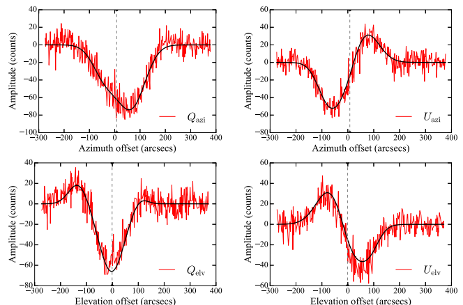
Fig. 3: Stokes Q_{\text{azi,elv}} (left column) and U_{\text{azi,elv}} (right column) data sets recorded at 4.85 GHz for the unpolarized, point-like source NGC 7027 in the two scanning directions, the azimuth in the top and the elevation in the bottom row. Instead of the expected flat, noise-like pattern, the presence of spurious signals are clearly visible in both scanning directions. The instrumental polarization, calculated by the instrument model M , is shown in each panel with a smooth black line. The dashed grey lines mark the source position along the scanning direction.
