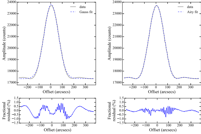
Fig. 7: A comparison between the Gaussian (left column) and Airy disk (right column) beam pattern models. The recorded data sets are shown in the top row with thick, grey lines and the model fits, with dashed, blue lines. The corresponding fractional residuals, (data-model)/data , are given in the bottom row for a direct comparison between the models.
