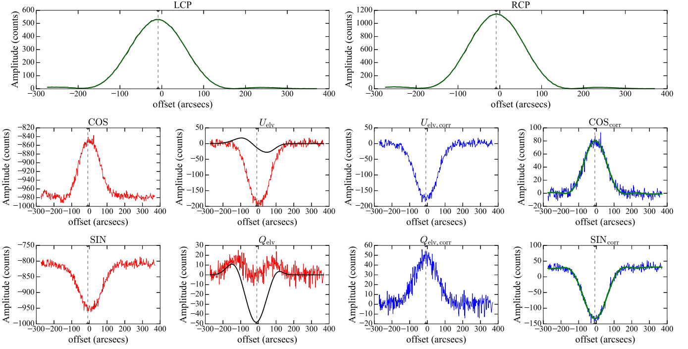
Fig. 5: Example of the instrumental linear polarization correction for an elevation sub-scan at 4.85 GHz. The observed COS/SIN (or equivalently Q_{\text{elv}}/U_{\text{elv}} ) signals are shown in the middle and bottom rows, right below the LCP signal (with red), while the corrected signals are shown right below the RCP signal (with blue). The correction is performed by subtracting the expected instrumental polarization signals (smooth black lines) from the observed Q_{\text{elv}} and U_{\text{elv}} data sets (2nd and 3rd column of the middle and bottom rows). The instrumental polarization signals are calculated by substituting the measured mean amplitude, I , peak offset, x and FWHM, \sigma , of the LCP and RCP signals (top row) in the instrument model, M , created for the given observing session.
