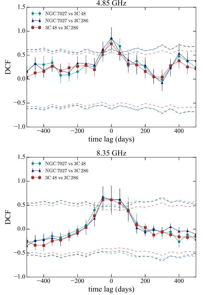
Fig. 14: Discrete correlation function (DCF) between the m'_c light curves of all source pairs including NGC 7027 and 3C 48 and 3C 286. The most prominent maxima above the 5\sigma significance levels, indicated by the corresponding dashed lines, appear around zero time lag where the correlation factor is \sim 0.8 \pm 0.2 and \sim 0.6 \pm 0.2 for the 4.85 GHz and 8.35 GHz data, respectively. The dashed lines indicate the 5\sigma significance level.
