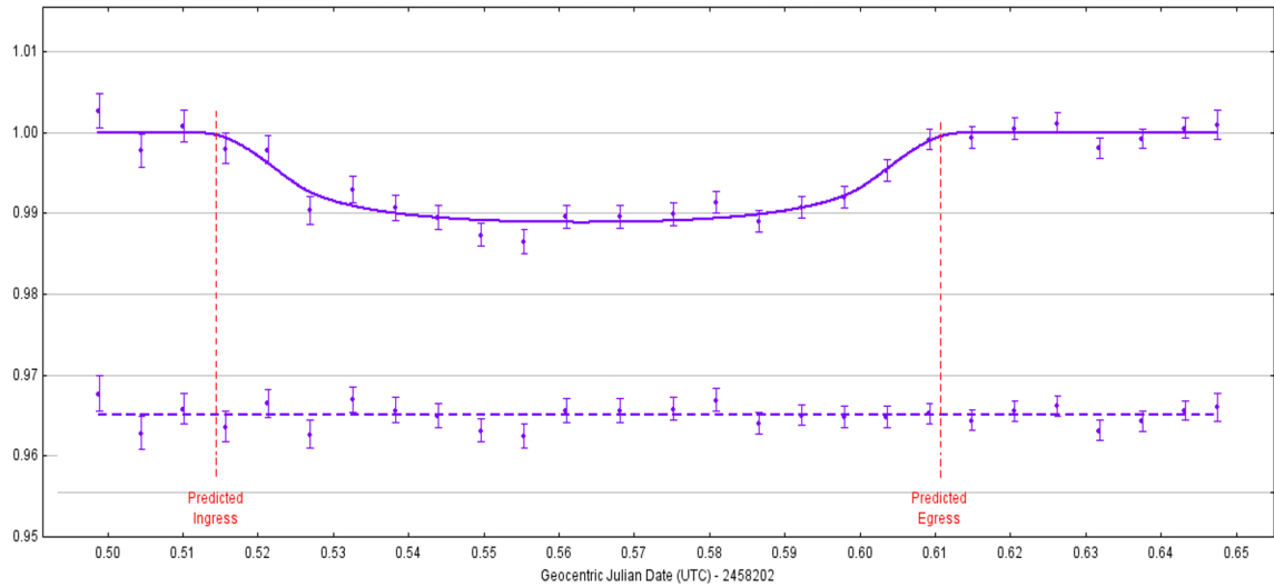
Figure 8. Light curve of Kepler-41b as observed at OPC the 25th of March 2018 with a low altitude field ( 30^\circ ). Each point represents 480 seconds of exposure and the S/N ratio is getting close to the size of the transit depth as expected.
