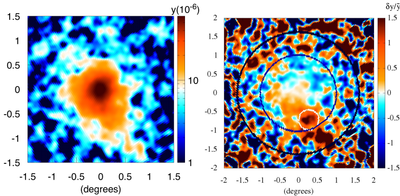
Figure 5: Left: The Planck y -map of the Coma cluster. Right: Residuals after subtracting the average Compton y profile, used to place constraints on the turbulent Mach numbers in the cluster outskirts via tSZ effect power spectral fluctuations [79].
