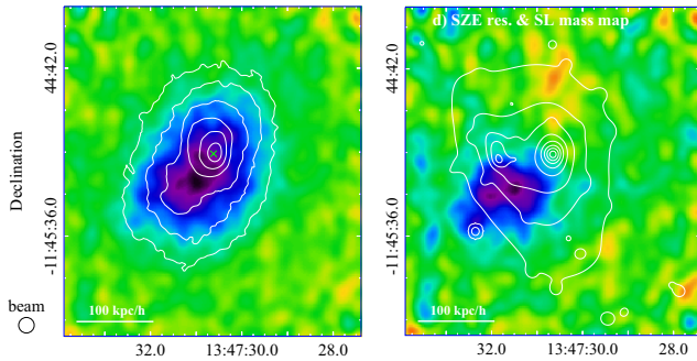
Figure 2: Left: ALMA+ACA image ( \sim 5'' resolution) of RX J1347.5-1145 with X-ray contours overlaid. Right: Substructure in the tSZ effect signal revealed after subtraction of a mean profile excluding the SE quadrant. Lensing contours are overlaid, revealing the location of the dark matter component. Figures from [23].
