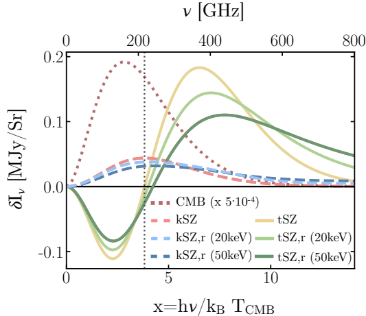
Figure 1: The tSZ (solid) and kSZ (dashed) effects, including relativistic corrections for various electron temperatures. The plots show the SZ effect distortions \delta I_{\nu} for different scenarios and compositions as a function of (dimensionless) frequency \nu ( x = h\nu/k_B T_{\text{CMB}} ), assuming an optical depth \tau_e = 10^{-2} , a Compton parameter y = 10^{-4} , and a line-of-sight peculiar velocity v_z = +1000 \text{ km s}^{-1} (typical of a massive galaxy cluster). The dotted, dark red curve illustrates the Planckian shape of the primary CMB spectrum scaled by a factor of 5 \times 10^{-4} for comparison purposes. Figure from [8].
