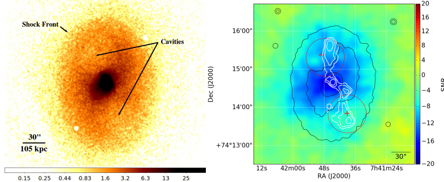
Figure 3: Chandra X-ray (left) and CARMA 30 GHz S/N (right) maps of MS0735.6. White contours on right delineate the radio bubbles; black are from X-ray, showing the cavity positions. Panels from [27, 32].
