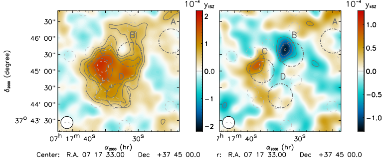
Figure 4: NIKA constraints on MACS J0717.5, using 150 & 260 GHz to reconstruct the tSZ (left) and kSZ (right) effect signals and to clean for contaminants. The tSZ effect map reveals T_e \gtrsim 18 keV gas, while the kSZ effect map reveals gas with v_z \approx 3000 km/s. Figures are from [73].
