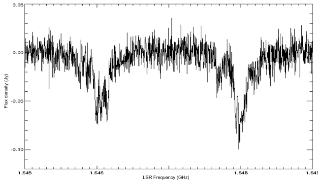
Figure 1. Spectrum of the galaxy NGC 5793 obtained with the GBT. The absorption lines are produced by the OH molecule at 1665 and 1667 MHz.
