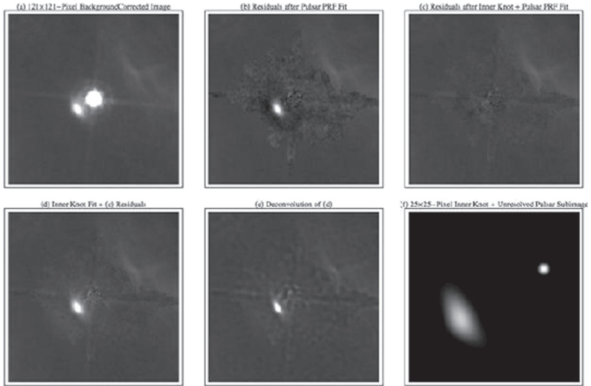
Figure 13. Images further illustrating steps in processing HST /ACS images of the Crab pulsar and inner knot: (a) subtract a linear-gradient background in the central 121 \times 121 pixel ( 6''.05 \times 6''.05 ) image of the pulsar and inner knot; (b) remove the pulsar using SVD model of PSF leaving inner knot; (c) remove the inner knot using its SVD model leaving residual background; (d) add the SVD model of the inner knot to the residual background; (e) apply the Richardson–Lucy algorithm to generate a deconvolved image of the inner knot (and residual background); and (f) synthesize the 25 \times 25 pixel ( 1''.25 \times 1''.25 ) sub-image of the registered (unresolved) pulsar and SVD model of the inner knot.
