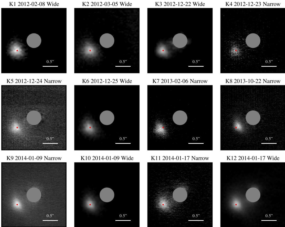
Figure 1. Individual images of the inner knot, with the pulsar removed, from Keck NIRC2 with laser guide star adaptive optics (AO). In each image, the PSF of the pulsar has been subtracted using the scaled PSF of a nearby star and replaced with a gray circle at the original location of the pulsar. Each image is 2'' \times 2'' . The images are from the NIRC2-wide camera ( 0''.04 pixels) or the NIRC2-narrow camera ( 0''.01 pixels). All images were taken using the K' filter. For positional reference, the red dot marks the average position of the inner knot across all 12 observations.
