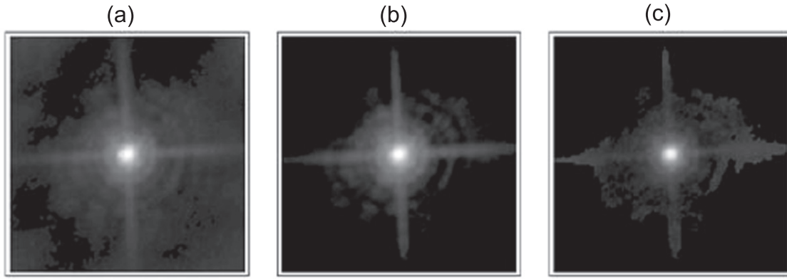
Figure 12. Images illustrating the steps in determining the HST /ACS PSF for this analysis: (a) extract 418 ( 19 \times 22 ) 121 \times 121 pixel ( 6''.05 \times 6''.05 ) images and subtract a linear-gradient background for 19 isolated stars in these 22 HST /ACS observations of the Crab; (b) register images of stars and use singular-value decomposition (SVD) to determine a basis describing the PSF (first SVD component shown); and (c) model the pulsar image using the first 72 SVD components.
