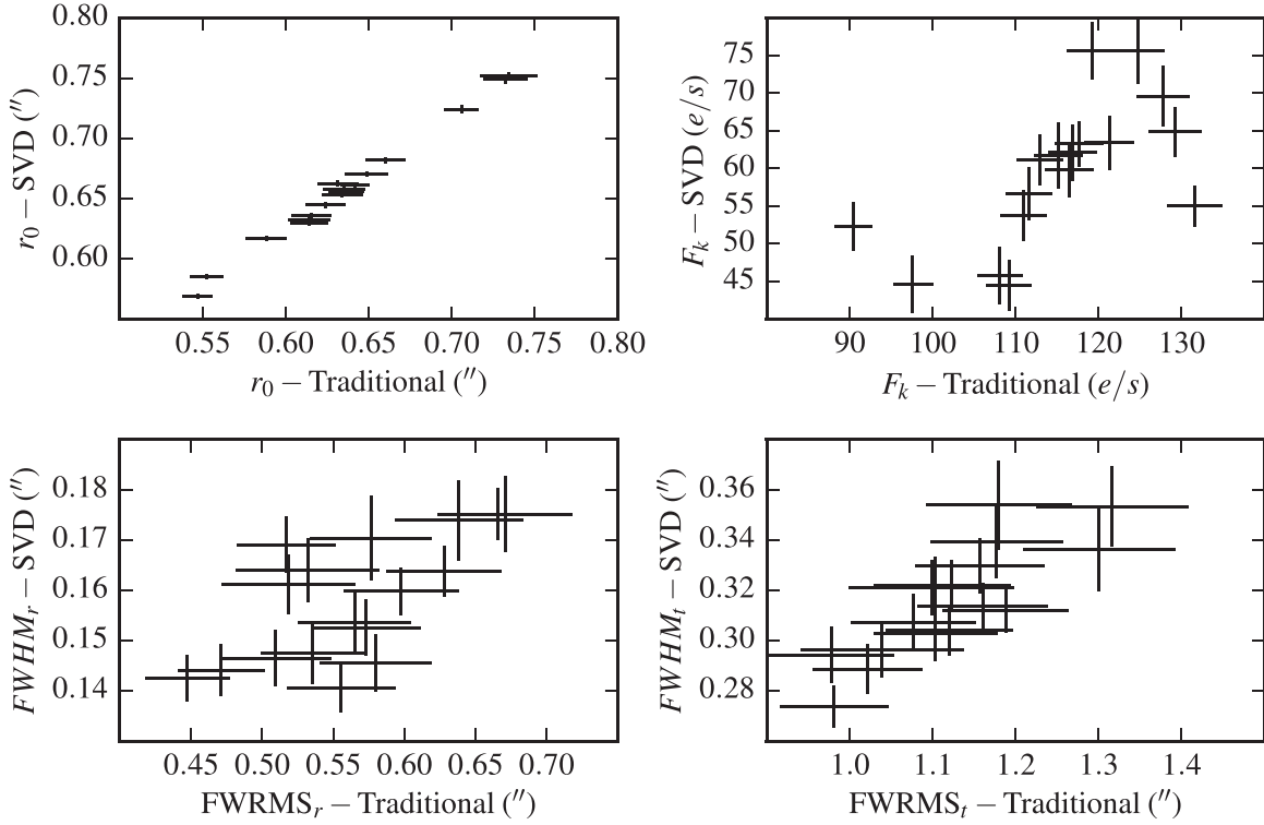
Figure 15. Comparison of HST -SVD and HST -traditional measured properties of the inner knot.
