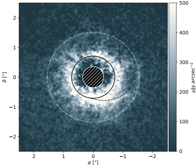
Fig. 2. Flux calibrated SPHERE/IRDIS DPI H -band observations ( Q_\phi image, in \mu\text{Jy.arcsec}^{-2} ), where we highlight the locations of the main and secondary belts, as well as the tentative spiral pattern.
