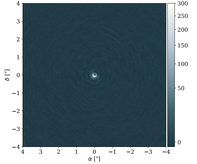
Fig. A.3. NACO L' image, with a square root scaling.
