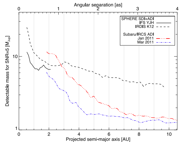
Figure 4. SPHERE sensitivity in mass to obtain a detection at SNR = 5 with the IFS (plain curve) and IRDIS (dashed curve), based on the injection of fake planets with spectra based on the BT-Settl synthetic spectra and evolutionary tracks (see Section 5.3 for details). These limits are compared to the contrast limits of Thalmann et al. (2011) in the Br \alpha filter at 4.05 \mu\text{m} that we converted into mass using the same set of models as for our SPHERE analysis. We discuss the comparison between the Subaru/IRCS and SPHERE/IRDIS limits in Section 6.
