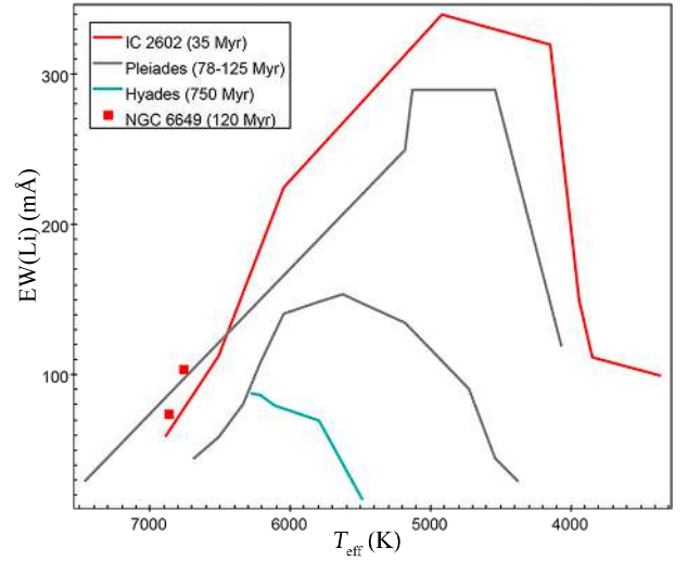
Fig. B.106. EW(Li)-versus- T_{\text{eff}} diagram for NGC 6649.
