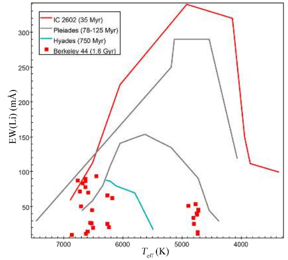
Fig. B.226. EW(Li)-versus- T_{\text{eff}} diagram for Berkeley 44.
