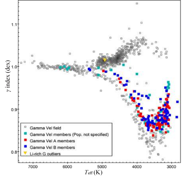
Fig. B.51. \gamma index-versus- T_{\text{eff}} diagram for \gamma Vel.
