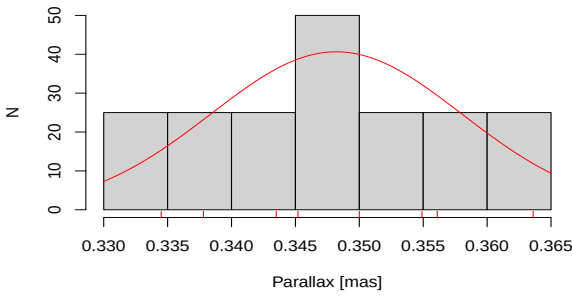
Fig. B.204. Parallax distribution for Melotte 71.
