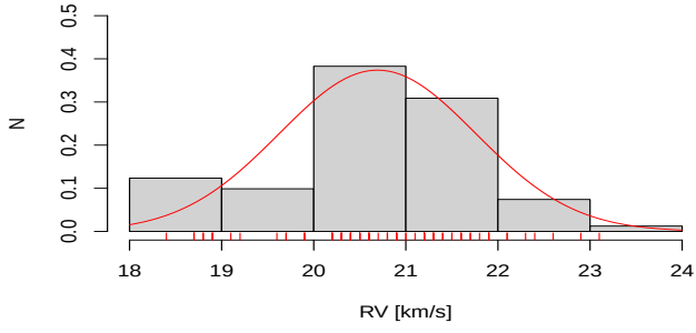
Fig. B.43. RV distribution for Col 197.
