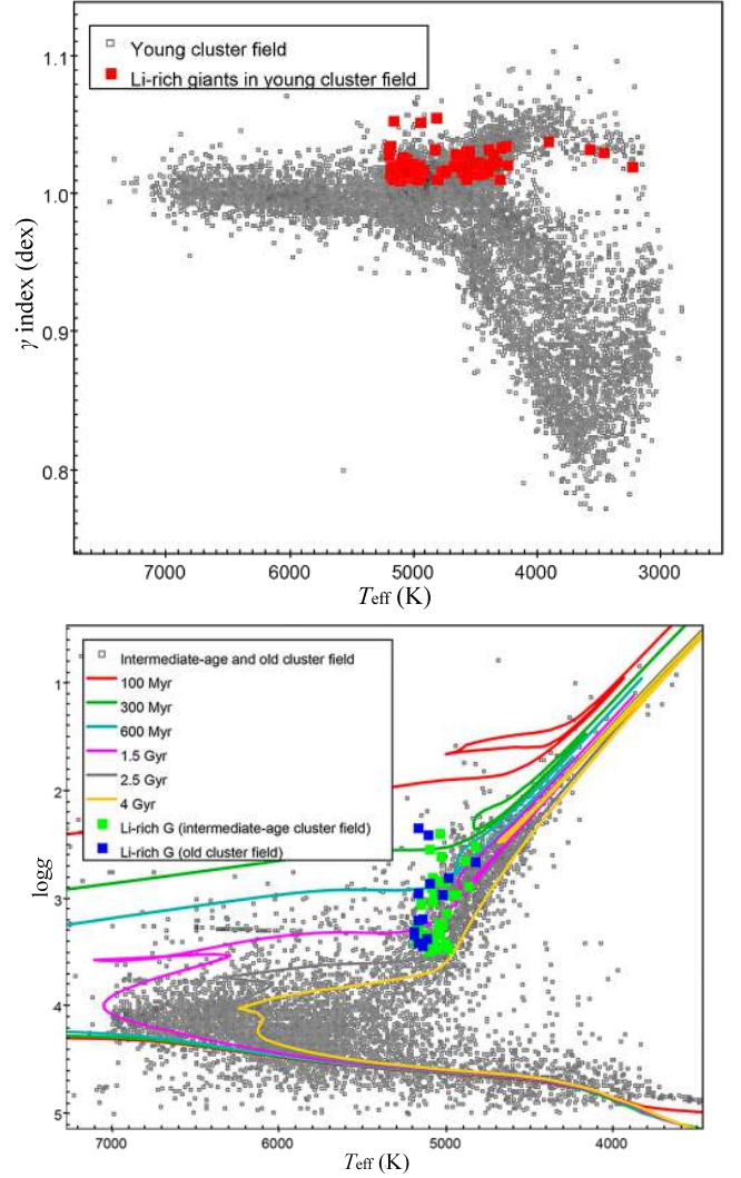
Fig. 5. \gamma index and \log g as a function of T_{\text{eff}} for the Li-rich giant outliers (red squares) in the field of the young (top), and intermediate-age (green squares), and old (blue squares) clusters (bottom).
