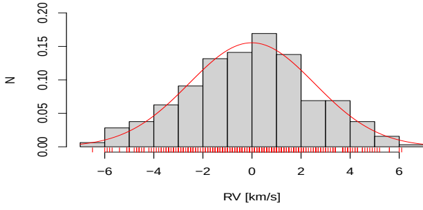
Fig. B.1. RV distribution for NGC 6530.
