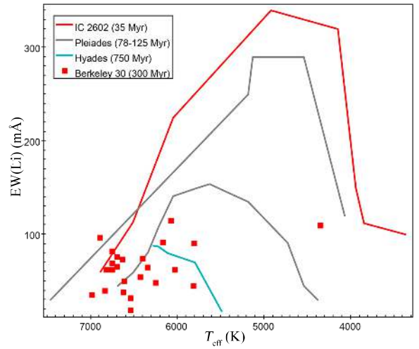
Fig. B.136. EW(Li)-versus- T_{\text{eff}} diagram for Berkeley 30.
