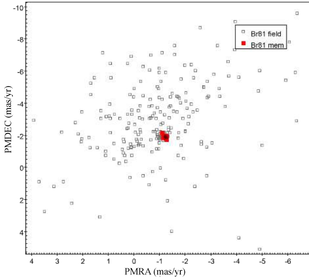
Fig. B.175. PMs diagram for Berkeley 81
