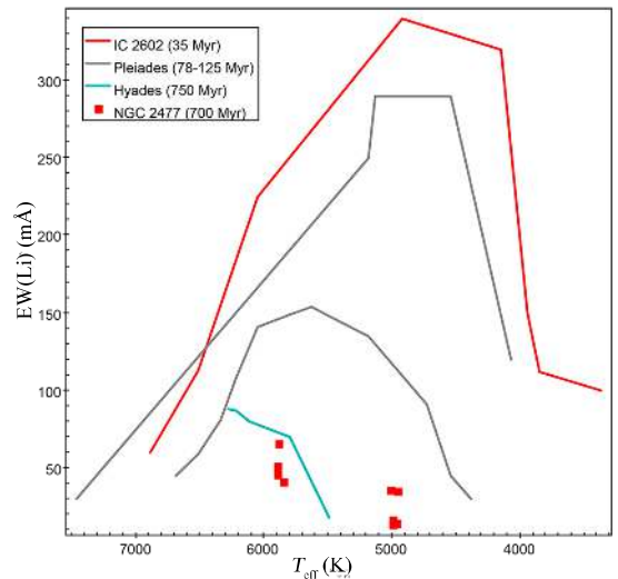
Fig. B.166. EW(Li)-versus- T_{\text{eff}} diagram for NGC 2477.
