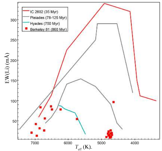
Fig. B.178. EW(Li)-versus- T_{\text{eff}} diagram for Berkeley 81.
