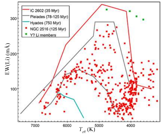
Fig. B.112. EW(Li)-versus- T_{\text{eff}} diagram for NGC 2516.
