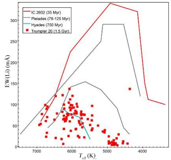
Fig. B.220. EW(Li)-versus- T_{\text{eff}} diagram for Trumpler 20.
