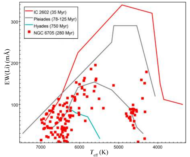
Fig. B.130. EW(Li)-versus- T_{\text{eff}} diagram for NGC 6705.
