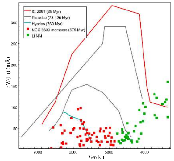
Fig. B.160. EW(Li)-versus- T_{\text{eff}} diagram for NGC 6633.
