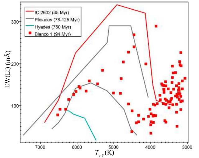
Fig. B.96. EW(Li)-versus- T_{\text{eff}} diagram for Blanco 1.
