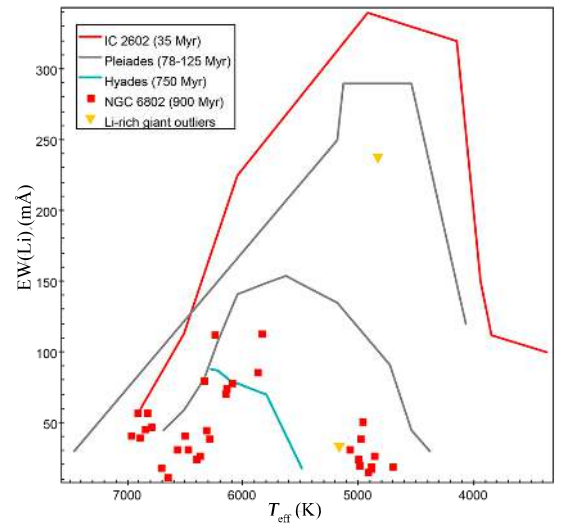
Fig. B.190. EW(Li)-versus- T_{\text{eff}} diagram for NGC 6802.
