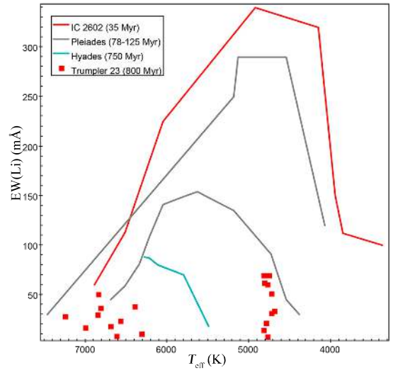
Fig. B.172. EW(Li)-versus- T_{\text{eff}} diagram for Trumpler 23.
