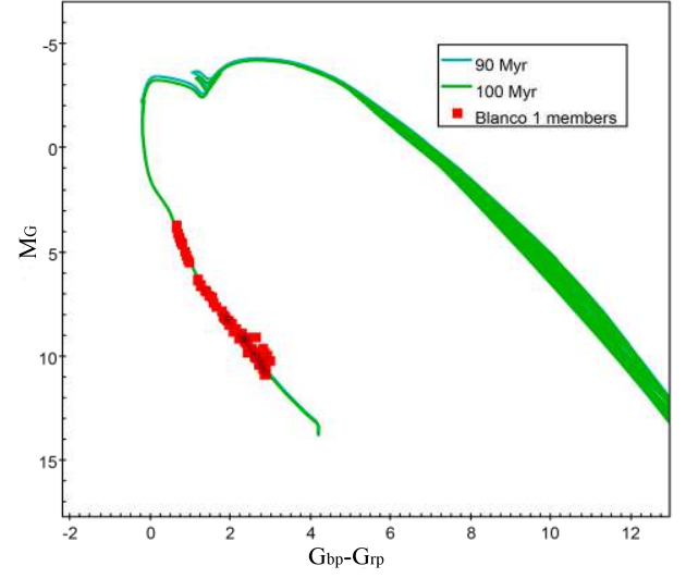
Fig. B.94. CMD for Blanco 1.
