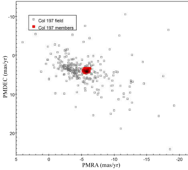
Fig. B.45. PMs diagram for Col 197.
