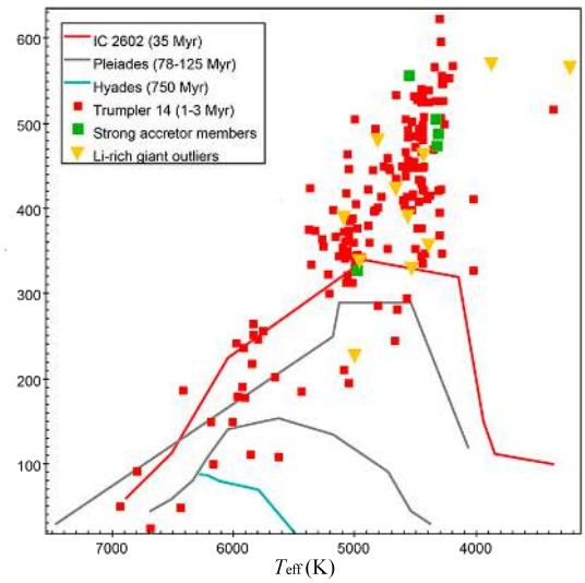
Fig. B.18. EW(Li)-versus- T_{\text{eff}} diagram for Trumpler 14.
