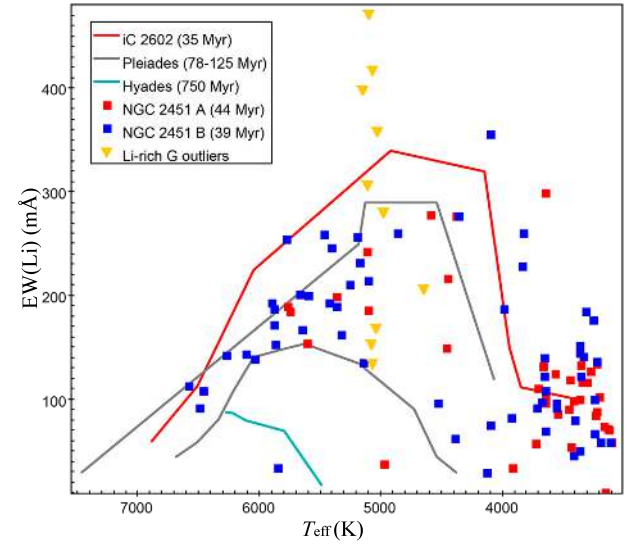
Fig. B.84. EW(Li)-versus- T_{\text{eff}} diagram for NGC 2451.
