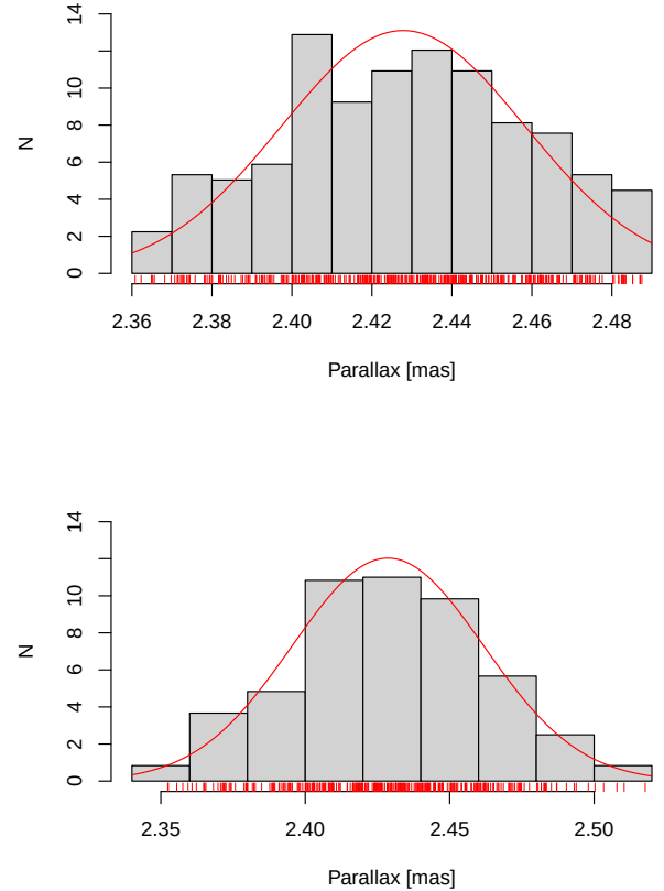
Fig. 2. Distributions of parallaxes and Gaussian fits for the intermediate-age cluster NGC 2516 (125–138 Myr). We display the histogram both for sources resulting from the 2\sigma clipping procedure on all the GES sources in this field (top panel), and for likely cluster members after applying all of our membership criteria (bottom panel).
