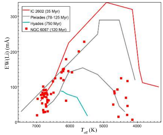
Fig. B.102. EW(Li)-versus- T_{\text{eff}} diagram for NGC 6067.
