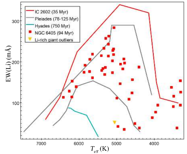
Fig. B.90. EW(Li)-versus- T_{\text{eff}} diagram for NGC 6405.
