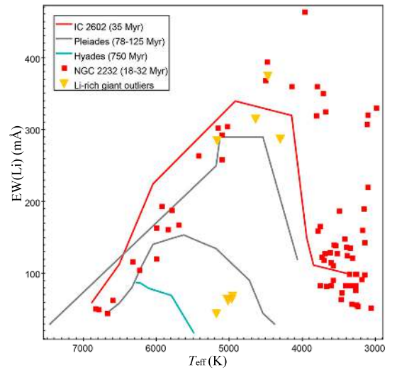
Fig. B.58. EW(Li)-versus- T_{\text{eff}} diagram for NGC 2232.
