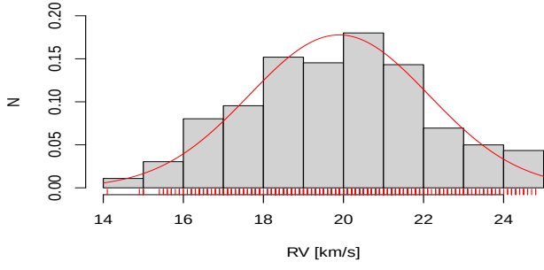
Fig. B.31. RV distribution for NGC 2264.
