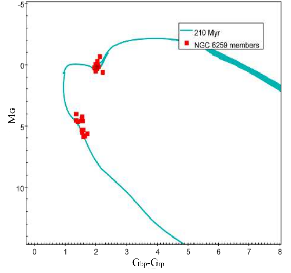
Fig. B.122. CMD for NGC 6259.
