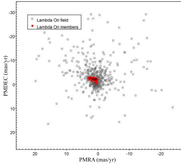
Fig. B.39. PMs diagram for \lambda Ori.
