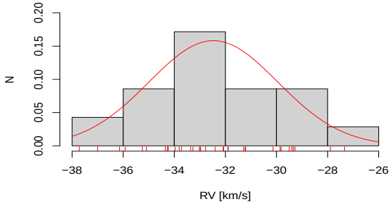
Fig. B.119. RV distribution for NGC 6259.
