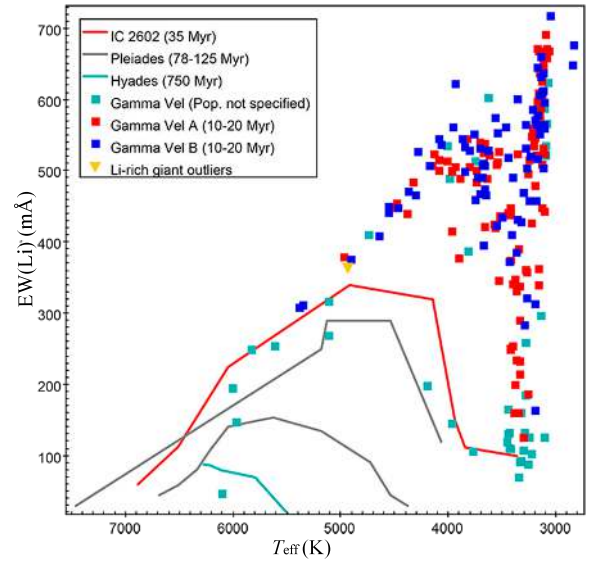
Fig. B.52. EW(Li)-versus- T_{\text{eff}} diagram for \gamma Vel.
