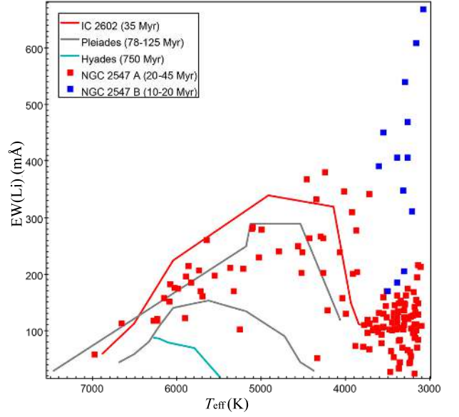
Fig. B.62. EW(Li)-versus- T_{\text{eff}} diagram for NGC 2547.
