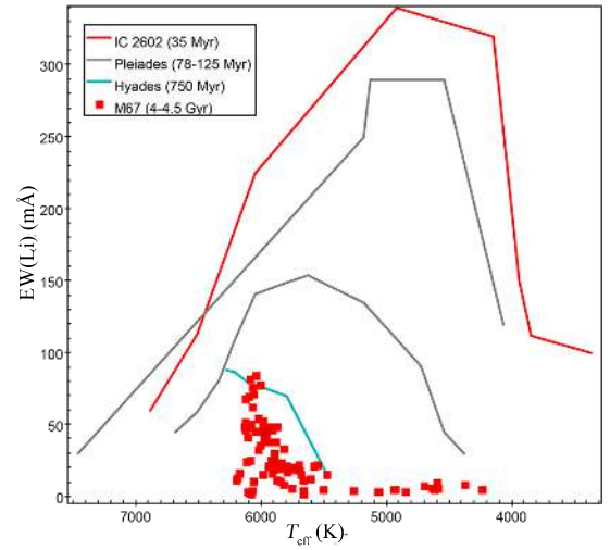
Fig. B.238. EW(Li)-versus- T_{\text{eff}} diagram for M67.
