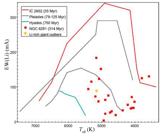
Fig. B.142. EW(Li)-versus- T_{\text{eff}} diagram for NGC 6281.
