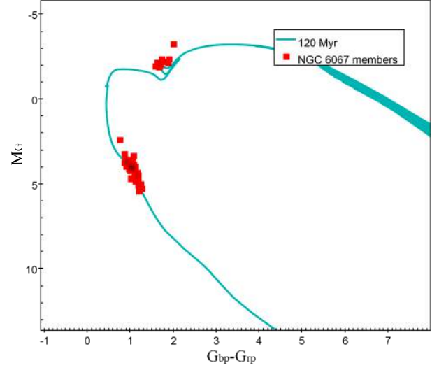
Fig. B.100. CMD for NGC 6067.
