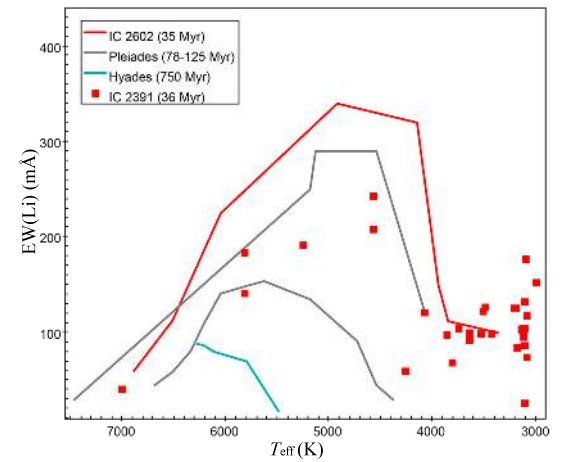
Fig. B.68. EW(Li)-versus- T_{\text{eff}} diagram for IC 2391.
