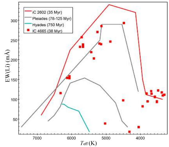
Fig. B.80. EW(Li)-versus- T_{\text{eff}} diagram for IC 4665.
