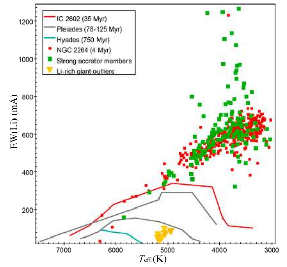
Fig. B.36. EW(Li)-versus- T_{\text{eff}} diagram for NGC 2264.
