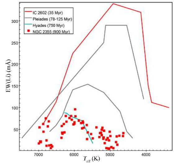
Fig. B.184. EW(Li)-versus- T_{\text{eff}} diagram for NGC 2355.
