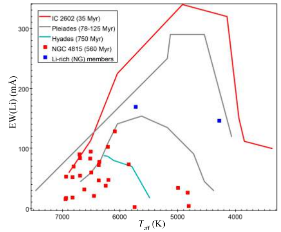
Fig. B.154. EW(Li)-versus- T_{\text{eff}} diagram for NGC 4815.
