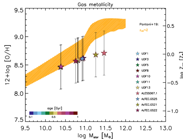
Figure 6. Statistical relationship between gas metallicity Z_{\text{gas}} and stellar mass M_{\star} for high- z star-forming progenitors of ETGs, by Pantoni et al. (2019) at z \sim 2 (orange), with its 1\sigma scatter (shaded area). Stars represent our outcomes for the 11 DSFGs of our sample derived as explained in Section 4.3. Symbols are colour-coded by the galaxy age (i.e. \tau_{\star} ).
