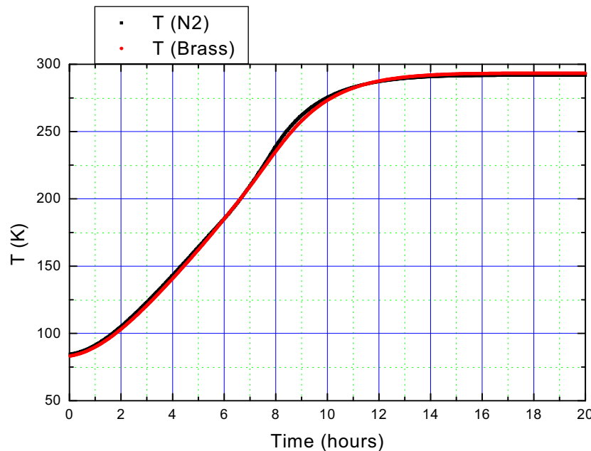
Figure 9 Time behavior in the heating of our cryogenic systems (experimental data)
