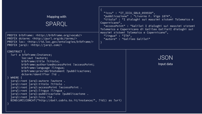
Fig. 2. JSON input and related JARQL mapping using SPARQL 1.1 syntax
