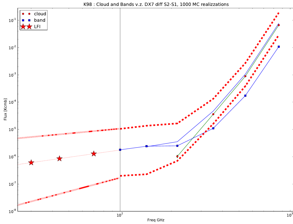
Figure 2: Sky averaged spectra in K_{\text{CMB}} of Zody and extrapolation at LFI Frequencies. The sky averaged signal for Cloud is denoted by circles, squares denotes the sky averaged signal for bands. Below 217 GHz the cloud signal is compatible with zero (the fit gives negative signal) so it can not be shown in this logarithmic plot. The line without symbols is the averaged sky signal, sum of Cloud and Bands. The two dashed red lines are T_{0,\text{zody},f} (bottom) and T_{\text{peak},\text{zody},f} (top). The stars represents the extrapolation of sky averaged signal at LFI frequencies.
