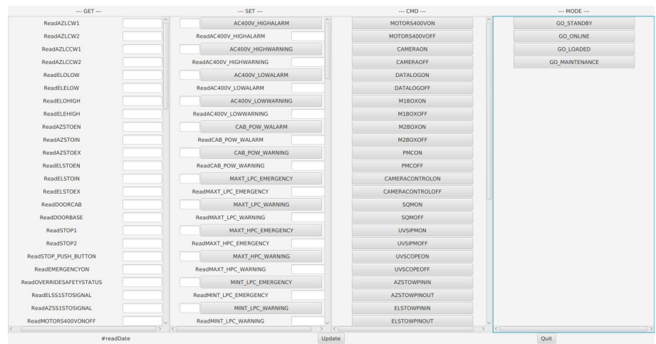
Figure 4: Generated GUI
