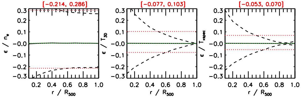
Fig. 3. Radial profiles of the relative uncertainties (\epsilon/Y - 1) on (left) gas density, (center) 3D gas temperature, and (right) projected spectroscopic-like temperature due to (i) the errors on the assumed parameters that describe the mass dependence, (ii) the scatter in the c - M - z relation, and (iii) the intrinsic scatter on the “universal” pressure profile. Red (green) dotted lines indicate the median values of the 16th and 84th percentiles (and of the medians) estimated at each radius. The case refers to the input values (M_{500}, z) = (4.6 \times 10^{14} M_{\odot}, 0.6) , which represents the median values of the S18 sample.
