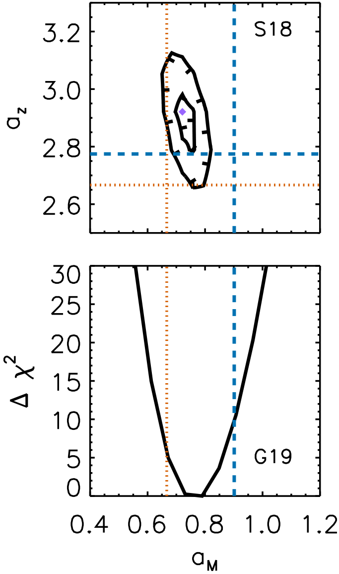
Fig. A.1. Constraints on the exponents a_M and a_z in P_\Delta \sim M^{a_M} E_z^{a_z} based upon the gas density and temperature profiles in S18 (top panel; likelihood contour at 1 and 5\sigma equivalent to \Delta\chi^2 of 6.2 and 28.8 for 2 degrees of freedom, respectively) and G19a (bottom panel; on a_M only, because all the 12 objects have a redshift <0.1 . For the sake of comparison, 5\sigma corresponds to \Delta\chi^2 of 25.0 for 1 degree of freedom). The dotted red lines are the predicted self-similar slopes, and the dashed blue lines correspond to the expected slopes from the i(\text{cm})z model.
