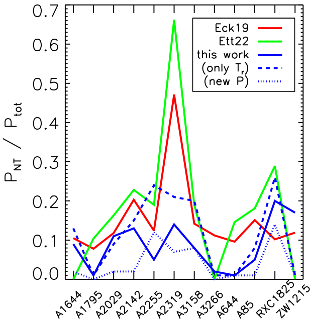
Fig. 7. Predicted 1\sigma upper limits on the value of the hydrostatic bias b here represented as the ratio between the nonthermal ( P_{NT} ) and total ( P_{tot} ) pressure in the ICM ( b = P_{NT}/P_{tot} ; see e.g., Eckert et al. 2019; Ettori & Eckert 2022). The dashed line represents the upper limit when only the temperature profile was used in the likelihood; when the new universal pressure profile also formed X-COP data (see Appendix B), the upper limits indicated with a dotted line were obtained. We note that the high level of nonthermal pressure support required for A2319 is explained by the ongoing merger described in Ghirardini et al. (2018).
