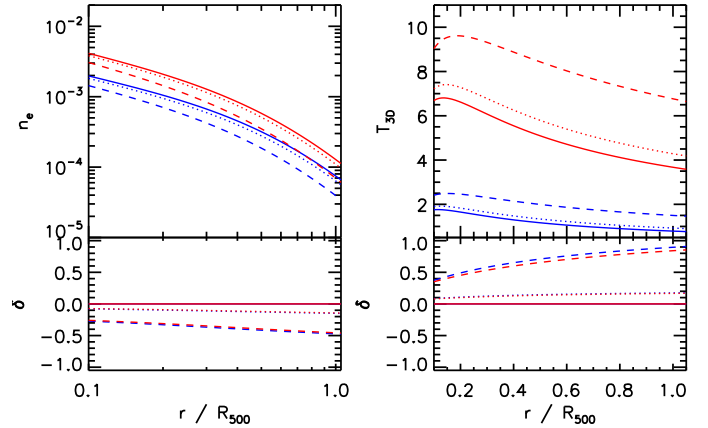
Fig. 6. Predicted electron density (left) and temperature (right) profiles of two halos at z = 0.05 and a hydrostatic mass M_{500} of 5 \times 10^{13} M_{\odot} (blue lines) and 5 \times 10^{14} M_{\odot} (red lines), respectively. Different line styles indicate the level of hydrostatic bias: b = 0 (solid lines); b = 0.2 (dotted line); and b = 0.6 (dashed line). Bottom panels: differences \delta = (M_b - M_0)/M_0 between the profiles with respect to the case with b = 0 .
