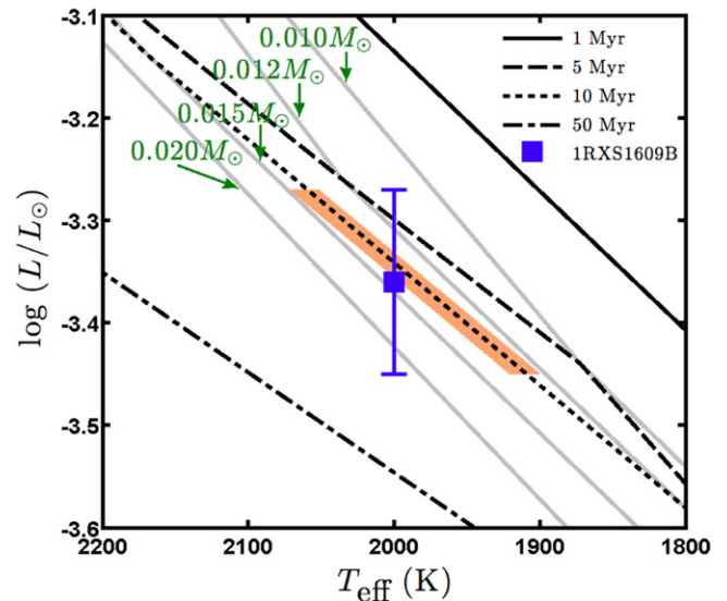
Figure 4. H-R diagram with DUSTY evolutionary tracks. Iso-mass curves are shown in gray. The salmon colored polygon is the only region consistent with the observed T_{eff} = 1900 – 2100 K, \log(L_{bol}/L_\odot) = -3.36 \pm 0.09 , and the age of Upper Sco ( 11 \pm 2 Myr). This yields a mass estimate of 0.012 – 0.015 M_\odot .
