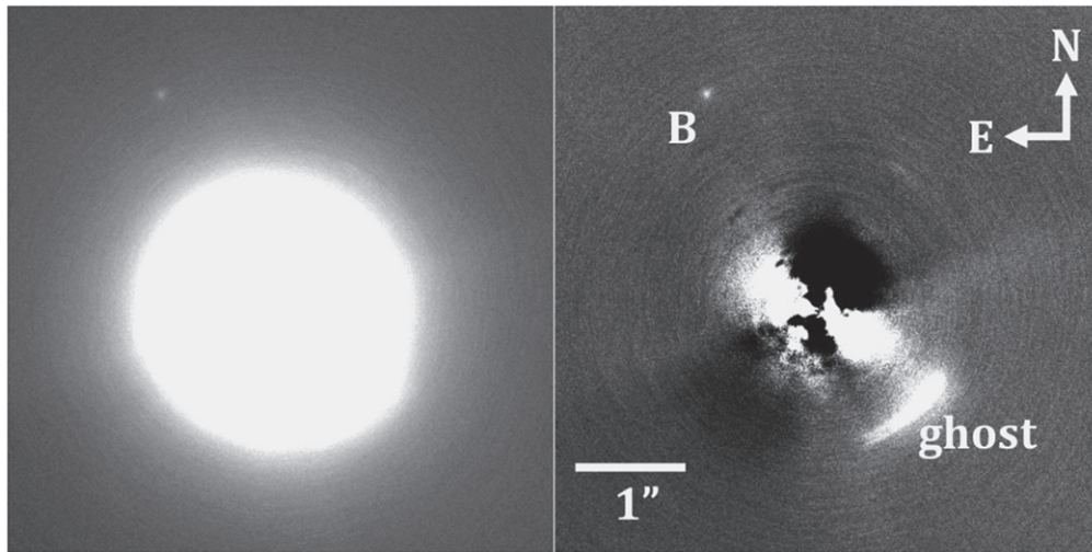
Figure 1. Left: 1RXS 1609 in MagAO z' filter. Right: after subtracting the radially symmetric profile of the primary star.
