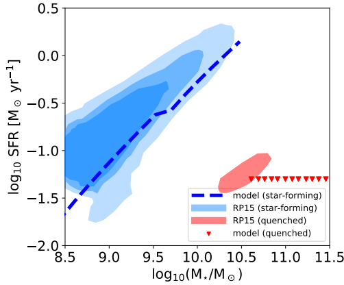
Figure 7. SFR averaged over the last 100 Myr vs M_{*} at z = 0 . The blue dashed line and the red triangles show galaxies from our fiducial model that are star-forming or quenched, respectively. The SFR of quenched system is set to an arbitrarily low value. The blue (red) shaded region shows the approximate distribution for star-forming (quenched) systems in SDSS from Renzini & Peng (2015) .
