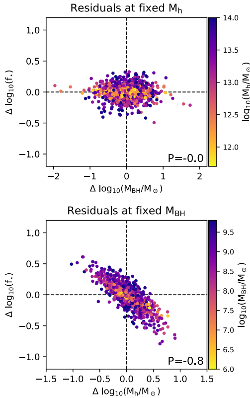
Figure 11. Residual correlation plot, analogous to that of Fig. 2, for a stochastic realisation of our fiducial model at z = 0 including a Gaussian scatter of 0.4 in \log(\epsilon_f) , \log(M_{\text{crit},0}/M_\odot) and \alpha . Only systems with M_h > 5 \times 10^{11} M_\odot and M_{\text{BH}} > 10^6 M_\odot are shown.
