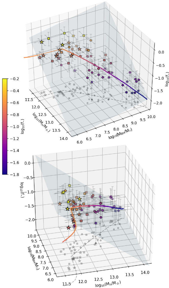
Figure 3. Two different 3D views for the distribution of our galaxy sample in the (M_h, M_{BH}, f_\star) space. The markers used in both panels are the same as in Fig. 1. The best-fit plane from eq. (1) is shown in dark grey. The 3D curve passing through the data shows the fiducial theoretical model from Section 4. To better enhance the 3D perspective, galaxies are colour-coded by their f_\star and 2D projections on the (M_h, M_{BH}) plane are shown.
