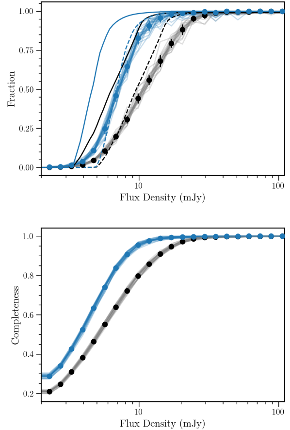
Fig. 10. Top: fraction of simulated sources detected as a function of flux density for each simulated image (in grey) and the median binned points (in black). The solid black line shows the fraction of sources that could be detected with a 5\sigma peak intensity threshold based on the rms only, while the dashed black line shows the same but assuming a single average smearing factor of 1.5, most applicable for the center of the field. The blue points and lines show the same, but determined only over the area with deep optical coverage. Bottom: Estimated completeness above a given flux density –assuming the 150-MHz source count distribution of Mandal et al. (2021)– scaled to 54 MHz assuming an average spectral index of -0.8 . This is estimated for the full field (shown in grey and black), and for the region of deep optical coverage (shown in light and solid blue).
