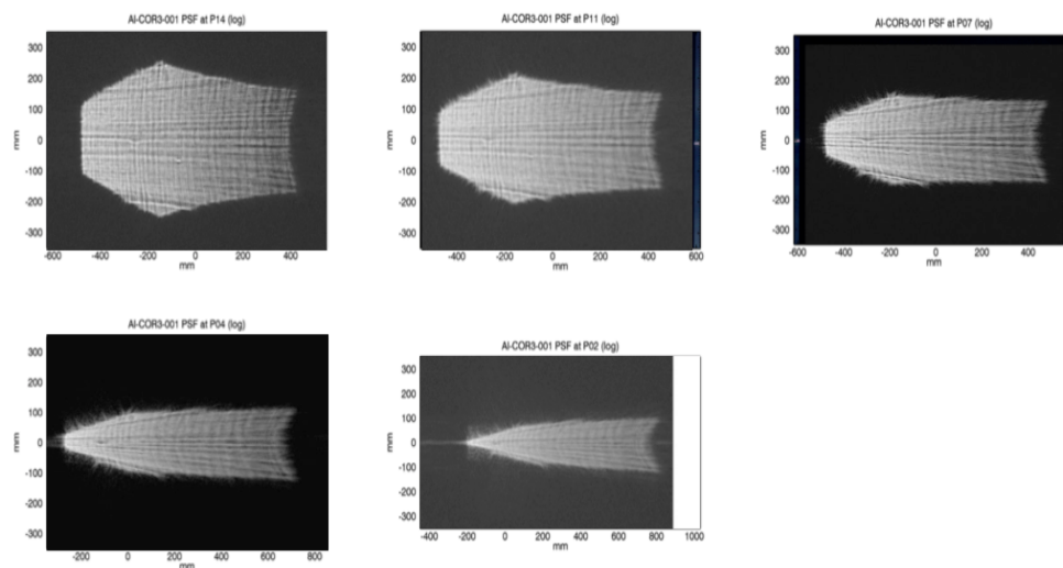
Figure 7. Image of the Pseudo-PSF of ASTRI-COR 3 segment simulated with the Physical Optics approach according to the setup described in Fig. 4: respectively from left to right \text{dist}_{\text{scr-mirr}} = 4761 \text{ mm} , 5794 \text{ mm} , 7059 \text{ mm} on the first row, and \text{dist}_{\text{scr-mirr}} = 8183 \text{ mm} , 8840 \text{ mm} on the second row.
