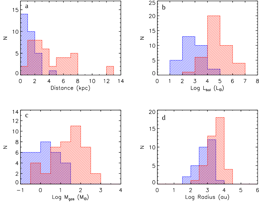
Fig. 5 Histograms of a ) distance, b ) bolometric luminosity, c ) gas mass of the circumstellar structure, and d ) outer radius of the circumstellar structure of the IM (blue) and HM (red) (proto)stars in Tables 1 and 2.
