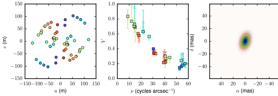
Fig. 11 The mid-IR geometry of the high-mass YSO V 921 Sco. Left panel: The uv-plane coverage of the VLT observations with the MIDI instrument. Middle panel: The visibility amplitude as a function of spatial frequency. The colour of the points corresponds with the position angle of the measurement. Right panel: Geometrical representation of the visibility function which consists of a compact 2D Gaussian combined with 1D Gaussian halo. Adapted from Boley et al. (2013).
