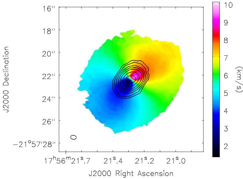
Fig. 7 Overlay of the 850 \mu\text{m} continuum emission ( contours ) on the CO (3–2) velocity map ( colours ) of the Keplerian disk around the Herbig Ae star HD 163296. From de Gregorio-Monsalvo et al. (2013).
