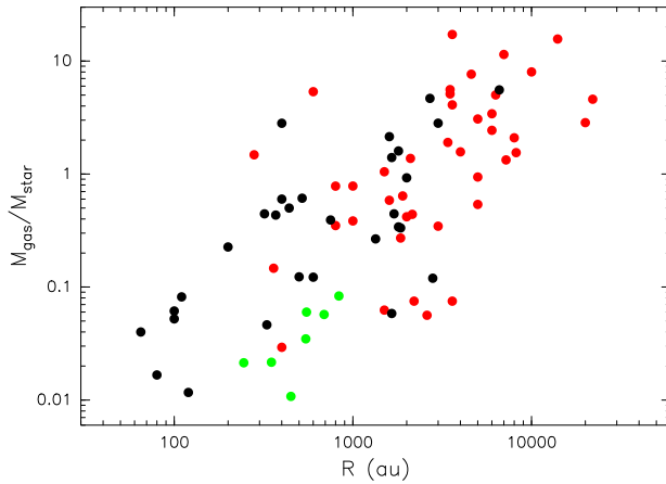
Fig. 8 Left panels: Gas mass to stellar mass ratio M_{\text{gas}}/M_{\star} as a function of the radius R of the circumstellar structures for the IM (black dots) protostars (Table 1) and the HM (red dots) (proto)stars (Table 2). Green dots correspond to Herbig Ae stars (see § 5.1.2).
