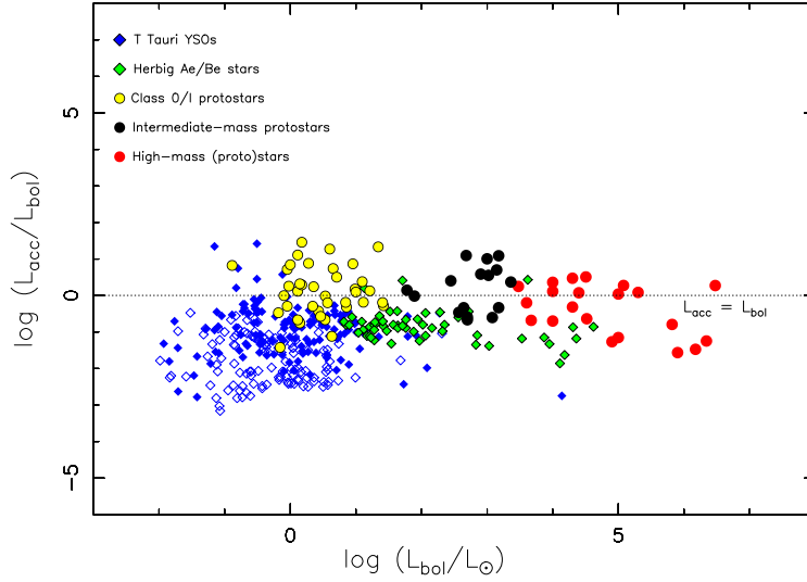
Fig. 18 Accretion luminosity L_{\text{acc}} to bolometric luminosity L_{\text{bol}} ratio as a function of L_{\text{bol}} for the same samples as in Fig. 17. Open symbols indicate upper limits.
