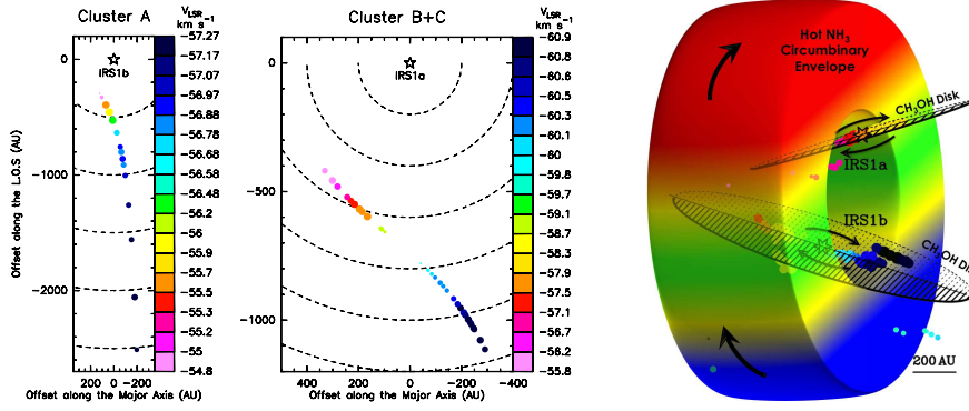
Fig. 10 Left panels: Estimated positions of individual 6.7 GHz CH 3 OH maser features towards the YSOs IRS1b and IRS1a in the high-mass star-forming region NGC7538 IRS1 derived from an edge-on disk model. The colours of the dots denote the maser velocity. Dashed arcs indicate circular orbits with radii increasing by steps of 500 and 200 au for IRS1b ( left ) and IRS1a ( right ), respectively. From Moscadelli & Goddi (2014). Right panel: Schematic model showing the nearly edge-on circumstellar rotating disks around IRS1a and IRS1b traced by the methanol maser emission surrounded by a circumbinary envelope traced in NH 3 . From Goddi et al. (2015)
