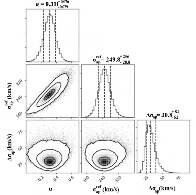
Fig. 6. Marginalized 2D and 1D posterior PDFs of the scaling relation parameters (slope \alpha , normalization \sigma_{ap}^{ref} , and intrinsic scatter \Delta\sigma_{ap} around the Faber-Jackson relation) obtained from fitting the measured velocity dispersions of 15 cluster galaxies. The dashed vertical lines in the histograms show the median and the 16-th and 84-th percentiles of the marginalized 1D distributions of each parameter. The parameter values are reported on the top of each figure.
