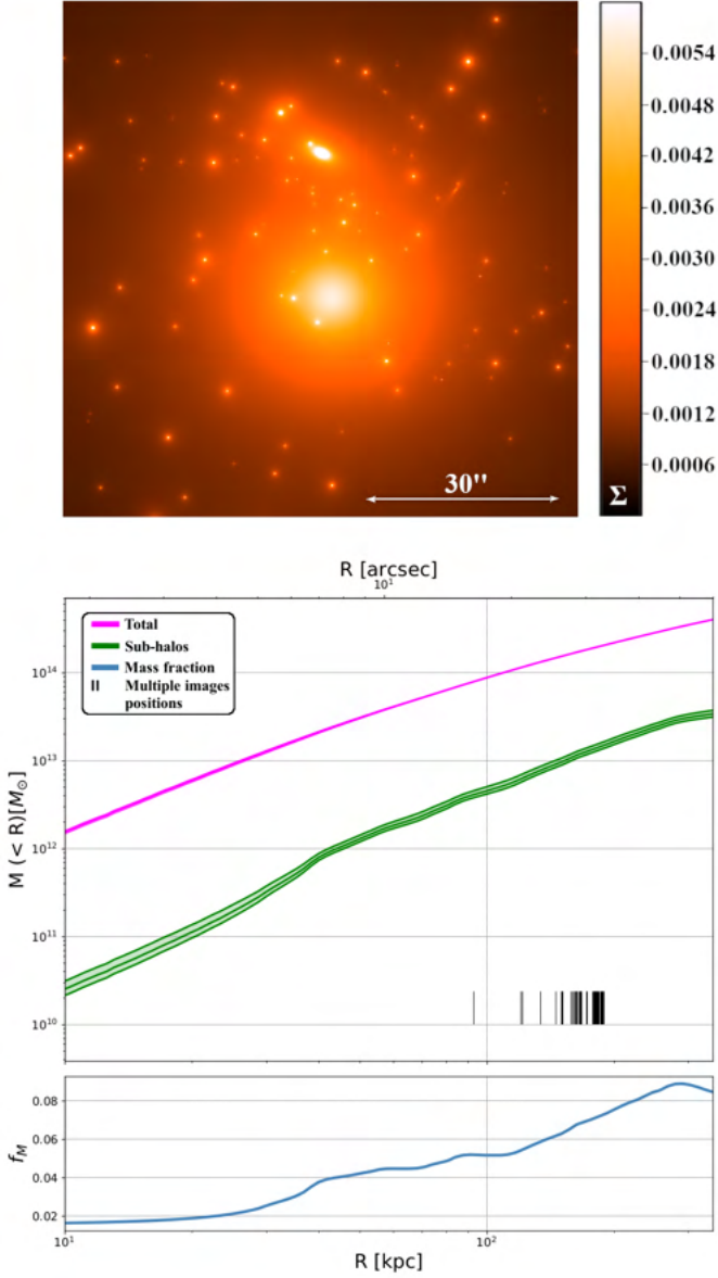
Fig. 10. Upper panel: Projected mass-density map for the reference model. The color scale is set between 0 and 0.006 in units of 10^{12} M_{\odot}/\text{kpc}^2 . Bottom panel: Projected cumulative mass profiles of PSZ1-G311 as a function of the projected distance from the BCG ( R ). In magenta we show the median value and the 1-\sigma confidence levels for the total mass profile. In green we show the median value and the 1-\sigma confidence levels for the subhalo component mass profile. The positions of the multiple images are marked with vertical black segments. The fractional contribution of the cluster member galaxies mass to the total cumulative mass is shown in blue.
