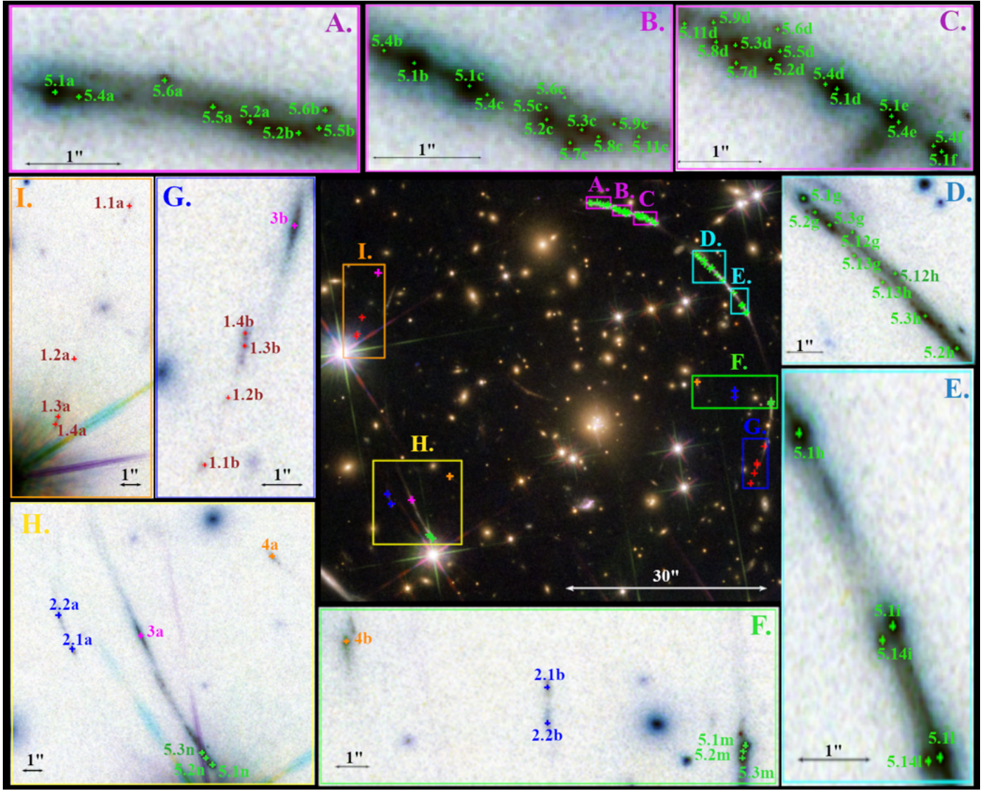
Fig. 1. HST color composite image of PSZ1-G311 with all cataloged multiple images shown. The first segment of the Sunburst Arc is highlighted in the magenta cut-outs A, B and C, and with the cyan cut-outs D and E, we can see almost all families of Sys-5, marked in green. Sys-1 (in red) is visible in both the orange (I) and blue (G) cut-out. In the latter we can also see family 3b, marked in magenta. Sys-2 (in blue) is visible in both the yellow (H) and green (F) cut-out. In cut-out H we can also see family 4a (in orange) and 3a, 5.1n, 5.2n, 5.3n. Images 4b, 5.1m, 5.2m, and 5.3m are visible in cut-out F.
