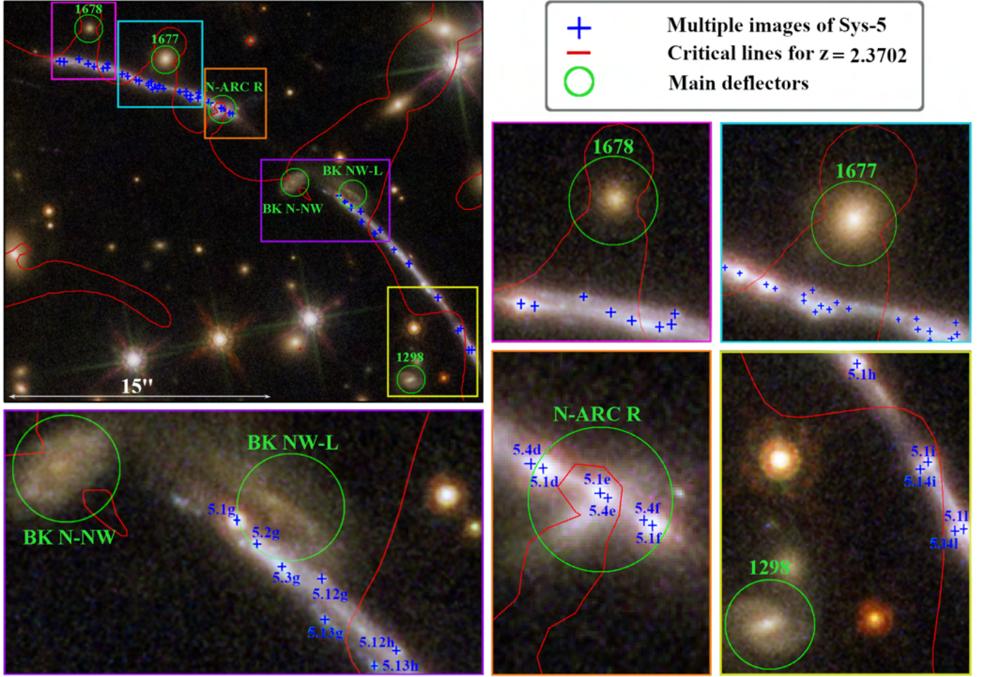
Fig. 7. The upper left panel shows a composite HST image of the two northern segments of the Sunburst Arc. The positions of the main deflectors are marked with green circles of radius 0.8'' . The regions indicated with colored rectangles around them are enlarged in the other panels. The multiple images of all families of knots belonging to Sys-5 are marked in blue, while the model-predicted critical lines are shown in red.
