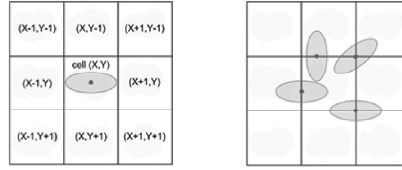
Figure 1. The C^3 sky partitioning method. The sky is partitioned in cells whose dimensions are determined by the maximum dimension that the matching regions can assume (panel a). Each source of the second catalogue is assigned to a cell; a source and an ellipse referred to a the first catalogue object can match only if the source lies within the nine cells surrounding the object (panel b).
