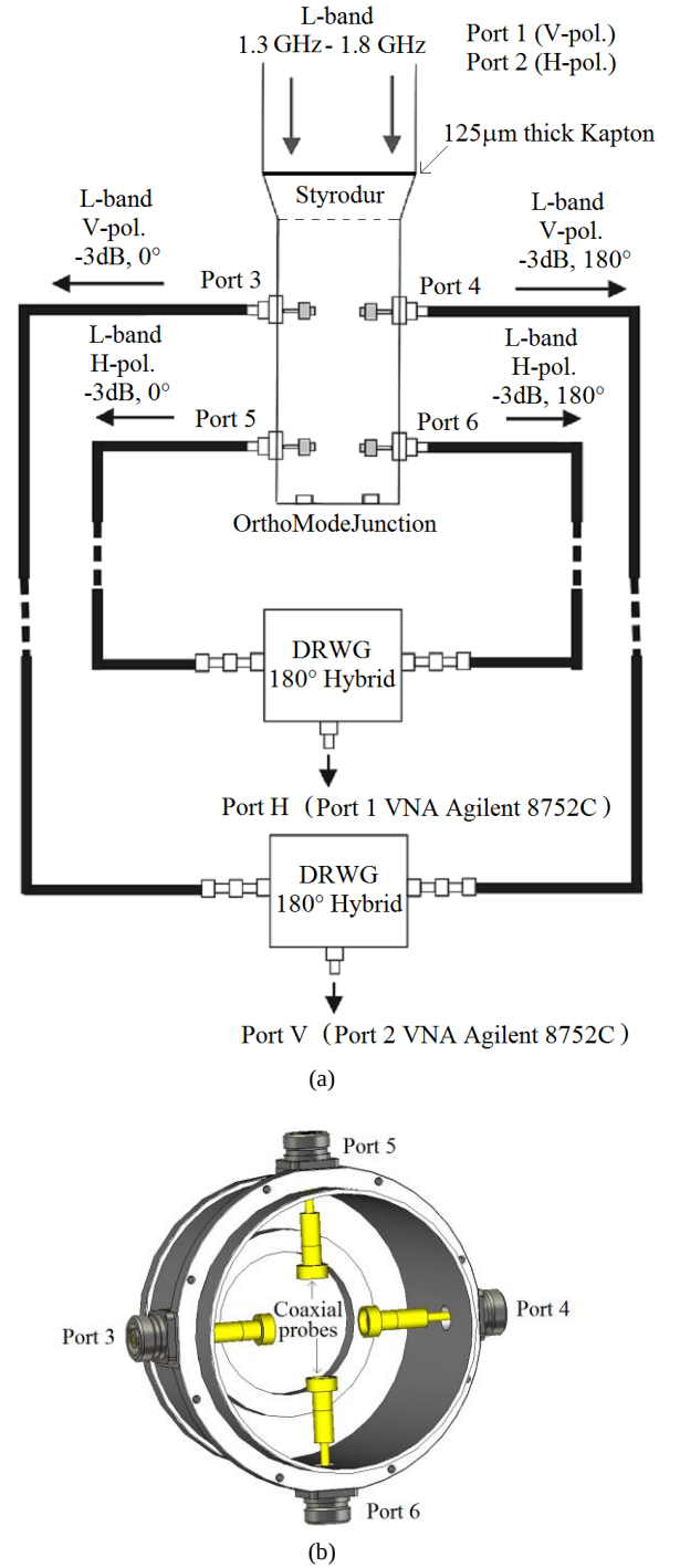
Fig. 1. (a) Sketch of the L-Band OMT showing the OrthoMode Junction, the two 180^\circ hybrids and the interconnecting cables. The two couples of probes are symmetrically disposed inside the OMJ but are depicted at different distance in the OMJ cavity for drawing clarity; (b) Internal detail of the OrthoMode Junction, showing the real configuration of the probes.
