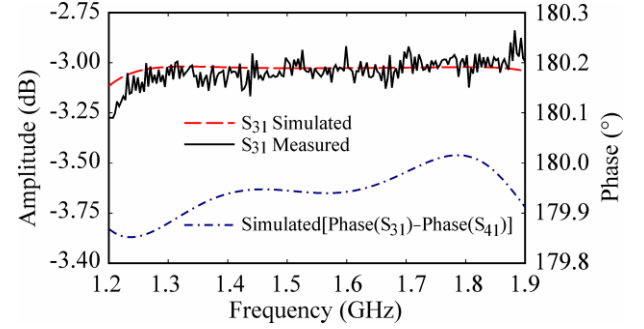
Fig. 8. Amplitude of the transmission coefficient S_{31} and simulated phase difference between the outputs at ports 3 and 4.
