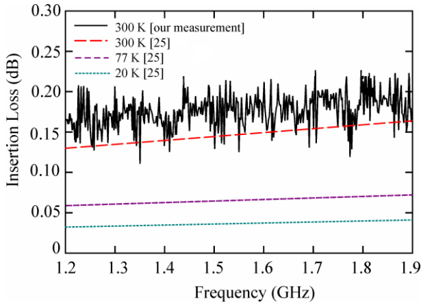
Fig. 17. Measured Insertion Loss of copper semi-rigid coaxial cables of length 350 mm at different temperatures.
