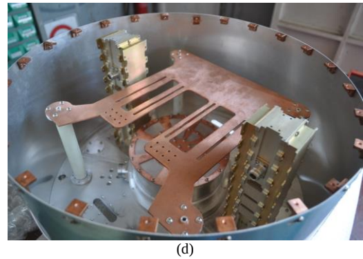
Fig. 3. Photos of fabricated OMJ prototype: (a) external view of the conical waveguide transition; (b) external view: detail of the circular waveguide section, circular waveguide-coaxial transitions, and air gap between stages 1 and 2; (c) internal view: detail of the coaxial probes; (d) internal view of the full orthomode transducer installed inside the cryostat.
