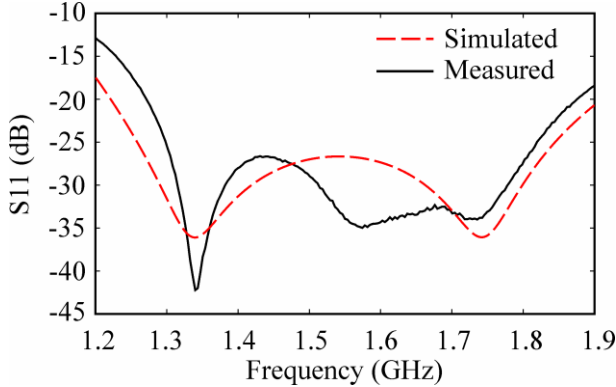
Fig. 7. Simulated and measured reflection coefficient ( S_{11} ) of the OMJ designed for operation across 1.3-1.8 GHz.
