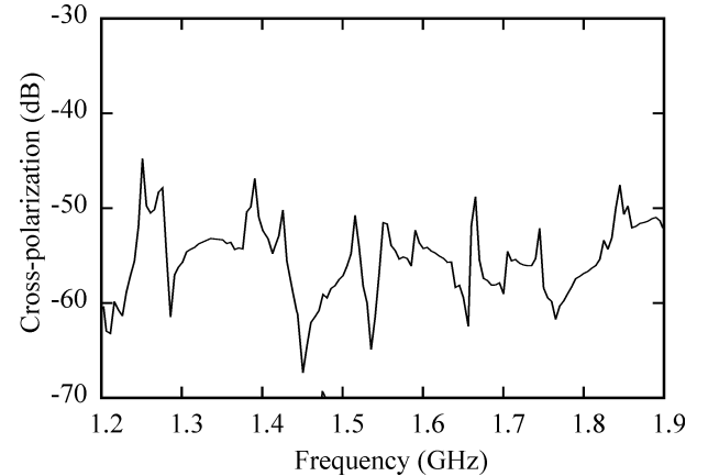
Fig. 9. Measured cross-polarization ( S_{51} ) of the OMJ.
