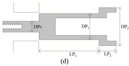
Fig. 2. (a) 3D view of the OMJ and DRWG 180° hybrids (supports for DRWG hybrids and coaxial cables between OMJ and hybrids are not shown); (b) 3D view of the OMJ and DRWG 180° hybrids: the DRWG Hybrids and the backshort of the OMJ are connected to copper plates @ 20K, the DRWG hybrids pass through holes in the aluminium plate at 77 K, without any contact with this plate; (c) cross-section of the OMJ; (d) detailed view of the OMJ coaxial probe.
