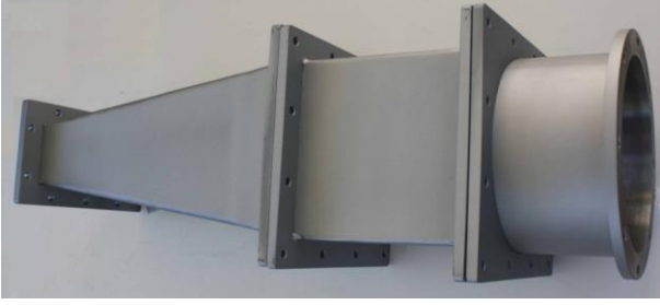
Fig. 5. Photo of the rectangular-to-circular waveguide transition consisting of three aligned mechanical parts. The flange on the rectangular side allows connection to the coaxial to rectangular transition. The flange on the circular side allows connection to the OMJ.
