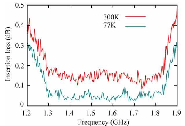
Fig. 16. Measured insertion loss of the DRWG Hybrid.
