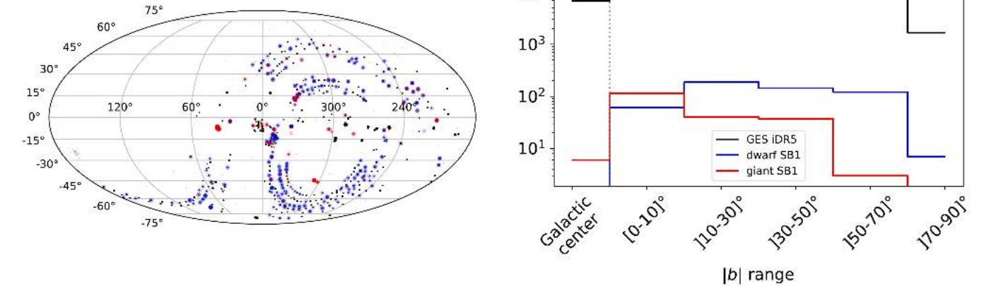
Fig. 14. Left: Mollweide projection of the GES iDR5 subsample (small grey pixels), with SB1 dwarf (large blue dots) and giant (large red dots) candidates from set 2 in Galactic coordinates. The darker a given region, the denser the observations in this region. Right: number of SB1 dwarfs (blue) and SB1 giants (red) within the specified Galactic latitude range excluding the Galactic centre. The first bin shows the same statistics but within 20° around the Galactic centre. GES iDR5 targets are also shown (black line).
