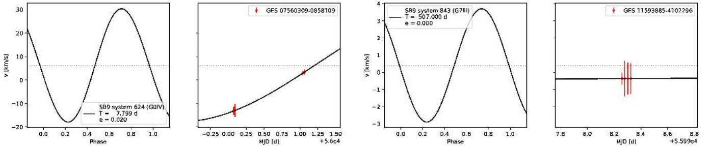
Fig. 18. Examples of Monte-Carlo simulations with (two left panels) and without (two right panels) detection of known circular SB1s from the SB9 catalogue. Red points represent simulated RV measurements at the epochs of a randomly chosen GES iDR5 target, with their estimated uncertainties. Spectral type, orbital period and eccentricity are indicated in the inset.
