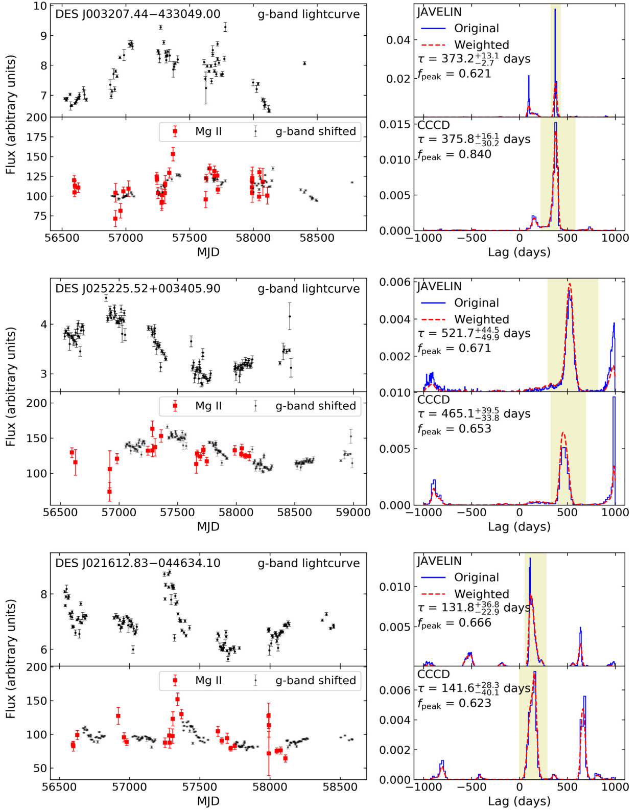
Figure 4. Light curves and lag measurements. Each 2 \times 2 grid of panels presents a source with the name shown in the upper left corner. (Left column) g-band continuum light curve and Mg II line light curve. The black points in the upper panel and the red squares in the lower panel represent the continuum and line light curve, respectively. The black points in the lower panel represent the continuum light curve shifted by the best-fitting JAVELIN lag. We re-scale the shifted continuum light curve so that its median matches the median of the line light curve. (Right column) JAVELIN and ICCF lag distributions. The blue solid lines in the upper and lower panels show the JAVELIN posterior lag distribution and the CCD from the ICCF method, respectively. The red dashed lines represent the weighted and smoothed lag distributions. The yellow shaded regions represent the ‘major peak’ ranges.
