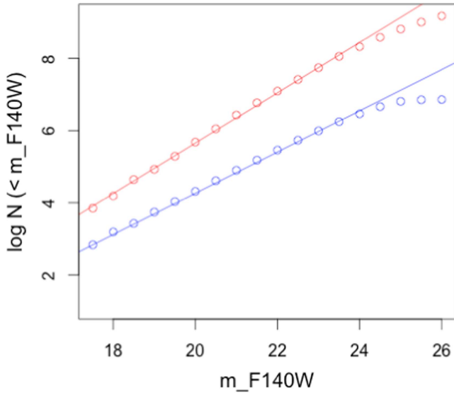
Figure 4. Log N -mag graph for our aggregated fields (blue dots) as well as the 3D- HST control sample (red dots). The y-axis is the logarithm of number of objects that have magnitudes less than or equal to the corresponding value on the x-axis. We fit the relationships for the region 19 < m_{\text{F140W}} < 24 with linear models and display the resulting fits (red and blue for 3D- HST and 3C samples respectively). We shift the 3CR data downward by 2 on the \log N(<m) axis (y-axis) in order to better display both sets of data, which otherwise overlap.
