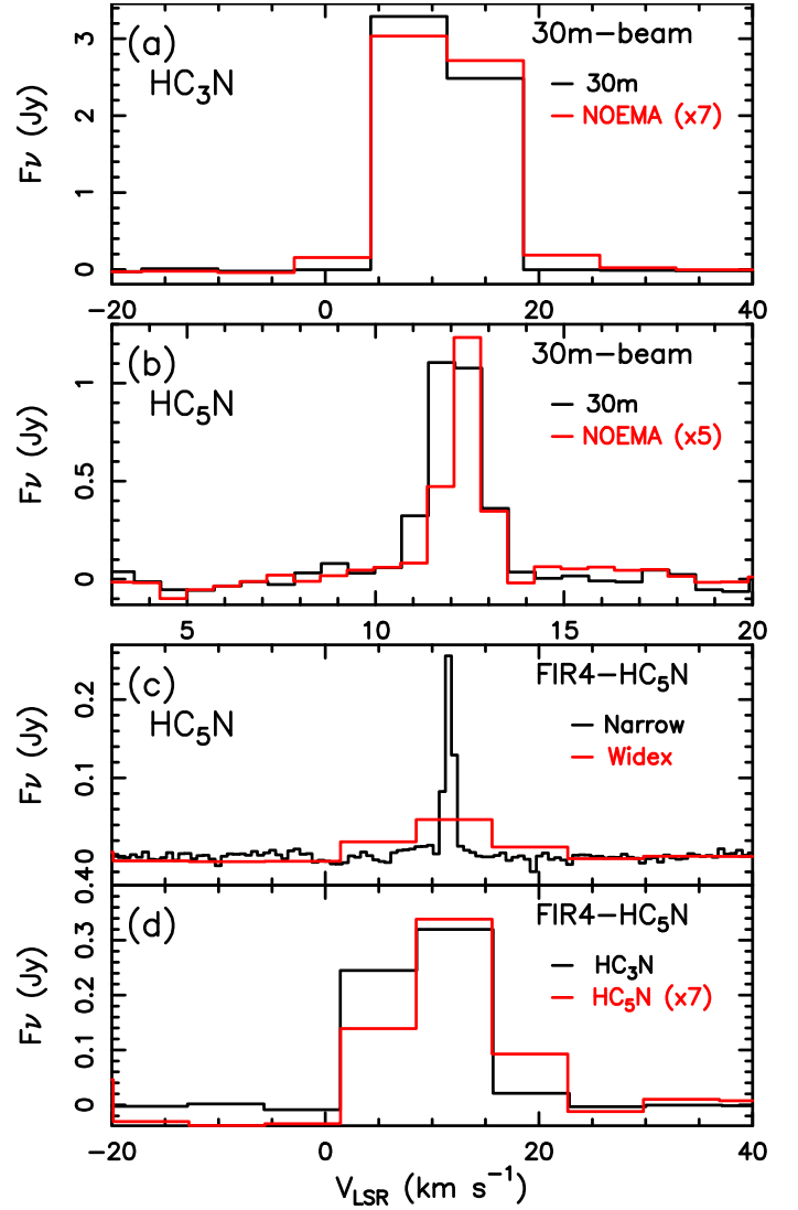
Fig. A.1. a) Spectrum of \text{HC}_3\text{N} (9–8) obtained with the IRAM-30 m Telescope (black histogram) in the framework of the ASAI large program, and SOLIS-NOEMA spectrum (red histogram) extracted from a circular region equal to the IRAM-30 m HPBW ( \sim 30'' ). We note that the flux resulting from the convolved NOEMA observations have been multiplied by a factor 7 to match those of the 30 m Telescope: we thus recover about the 15% of the total flux. b) Same as panel a for \text{HC}_5\text{N} (31–30). In this case, the NOEMA spectrum has been multiplied by a factor 5. From the plot, it is apparent that we recover slightly less than the 20% of the total flux. c) Comparison between the Narrow (black) and Widex (red) spectrum of \text{HC}_5\text{N} (31–30), both integrated on the region FIR4- \text{HC}_5\text{N} (red contour in Fig. 1). The integral under the channel with signal is different by \sim 7\% (see Sect. 2). d) Widex spectra of \text{HC}_3\text{N} (black) and \text{HC}_5\text{N} (red) integrated over the same region as in panel c. The \text{HC}_5\text{N} spectrum has been multiplied by 7 for clarity of the figure.
