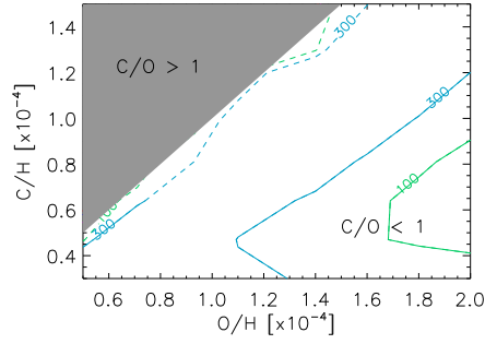
Fig. A.3. Predictions of the \text{HC}_3\text{N}/\text{HC}_5\text{N} abundance ratio from the chemical models described in Sect. 3.2 for \zeta = 1 \times 10^{-17} at the five different times (from top to bottom): 1 \times 10^4 yr, 3 \times 10^4 yr, 1 \times 10^5 yr, 3 \times 10^5 yr, and 1 \times 10^6 yr. All symbols used (contour plots, grey zone, etc.) are the same as in Fig. 3.
