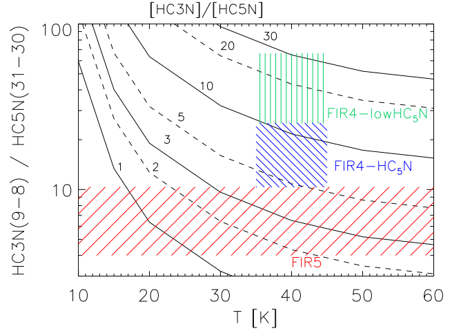
Fig. 2. Theoretical \text{HC}_3\text{N} (9–8)/ \text{HC}_5\text{N} (31–30) line intensity ratio assuming LTE and optically thin conditions as a function of the gas temperature for different values of the \text{HC}_3\text{N}/\text{HC}_5\text{N} abundance ratio as marked (black curves). The range of values observed within a 2\sigma error bar towards the three regions listed in Table 1 are showed as dashed areas: FIR4- \text{HC}_5\text{N} (blue), FIR4-low \text{HC}_5\text{N} (green) and FIR5 (red). We note that the temperature of FIR4 was estimated to be \sim 40 K (Ceccarelli et al. 2014) while no estimates for FIR5 exist.
