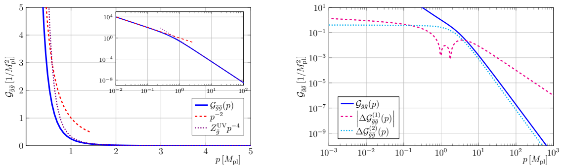
Figure 6: Momentum dependence of the Euclidean background graviton propagator \mathcal{G}_{\bar{g}\bar{g}}(p) . (left) Momentum dependence of the Euclidean background graviton propagator (blue, solid) with its IR and UV asymptotics. The UV asymptotic (violet, dotted) is given by p^{-4} with Z_{\bar{g}}^{\text{UV}} \approx 18.5 , see (25). The IR asymptotic (red, dashed) is simply the classical dispersion 1/p^2 . (right) Subleading contributions at small momenta in comparison to the full propagator (blue, solid). \Delta\mathcal{G}_{\bar{g}\bar{g}}^{(1)} (magenta, dashed) carries a subleading log-like contribution, while \Delta\mathcal{G}_{\bar{g}\bar{g}}^{(2)} (cyan, dotted) carries a constant contribution for small momenta.
