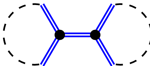
Figure 5: Tree-level graviton-graviton scattering diagram. The dashed lines indicate the transverse-traceless contraction of the external legs.
