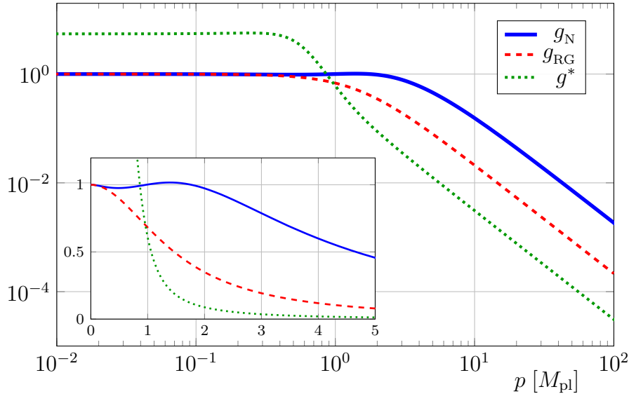
Figure 4: Physical Newton coupling g_N(p) = G_N(p)M_{\text{pl}}^2 as a function of momentum in units of the Planck mass (blue, solid). For comparison, we also show the scale-dependent Newton coupling g_{\text{RG}} = g_k(p=0) (red, dashed) as a function of k = p , and the fixed-point coupling g^*(p/k) as a function of a dimensionless momentum variable (green, dotted).
