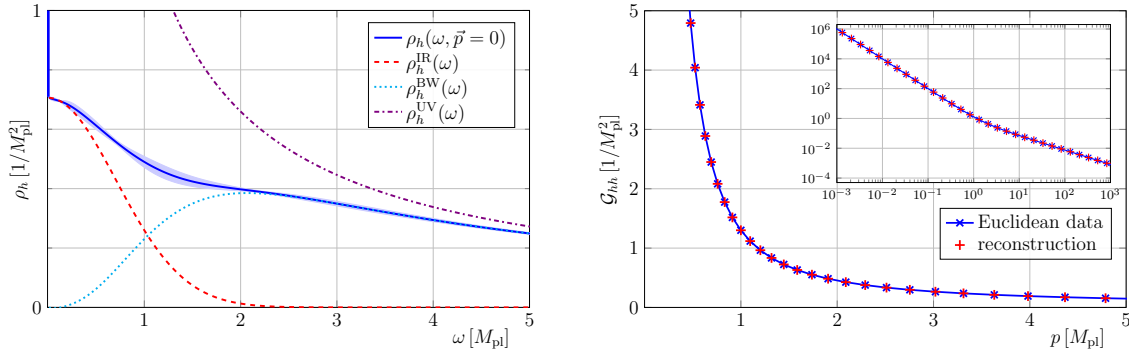
Figure 7: Spectral function of the fluctuation graviton and the reconstructed Euclidean propagator. The reconstruction, the definition of its error, and the error band in Sec. 5 are described in Sec. 5.1 and Sec. 5.2 . (left) Spectral function of the fluctuation graviton (blue, solid line). It features a \delta -function at \omega = 0 (massless graviton), and an ensuing smooth multi-particle continuum, \rho_h^{\text{cont}}(\omega) . We also depict the analytic IR- and UV-asymptotics (red, dashed and violet, dash-dotted), and the Breit-Wigner part (cyan, dotted). (right) Euclidean fluctuation propagator reconstructed from the spectral function presented in the left panel. The reconstructed and original Euclidean data agree very well on all data points corresponding to a reconstruction error of E_{\text{rel}} < 10^{-6} .
