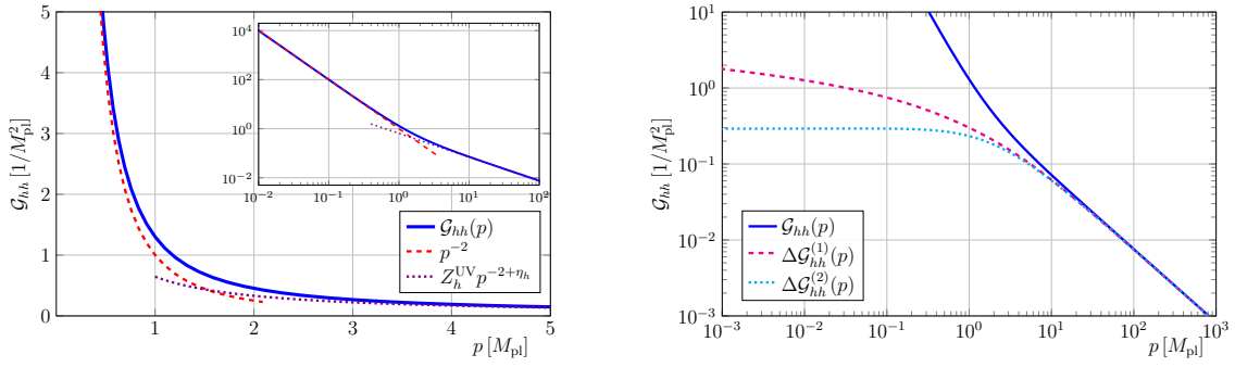
Figure 3: Momentum dependence of the Euclidean fluctuation graviton propagator \mathcal{G}_{hh}(p) . (left) Momentum dependence of the Euclidean fluctuation graviton propagator (blue, solid) with its IR and UV asymptotics. The UV asymptotic (violet, dotted) is given by Z_h^{\text{UV}} p^{-2+\eta_h} with \eta_h = 1.03 and Z_h^{\text{UV}} = 0.64 , see (25). The IR asymptotic (red, dashed) is simply the classical dispersion 1/p^2 . (right) Subleading contributions at small momenta in comparison to the full propagator (blue, solid). \Delta\mathcal{G}_{hh}^{(1)} (magenta, dashed) carries a subleading log-like contribution, while \Delta\mathcal{G}_{hh}^{(2)} (cyan, dotted) carries a constant contribution for small momenta.
