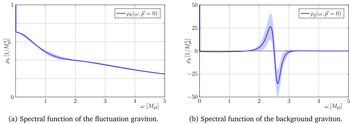
Figure 1: Spectral functions of the fluctuation and background graviton. The shaded areas constitute the estimated error of the reconstruction. The fluctuation graviton spectral function is strictly positive, which may be important for the unitarity of asymptotically safe gravity. In turn, we show that the background graviton spectral function has a vanishing spectral weight and hence positive and negative parts. For more details see Sec. 5.2 and Sec. 5.3 .
