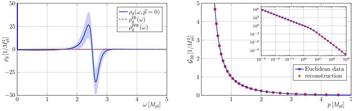
Figure 8: Spectral function of the background graviton and reconstructed Euclidean graviton propagator. The reconstruction, the definition of its error, and the error band in Sec. 5.1 are described in Sec. 5.1 and Sec. 5.3. (left) Spectral function of the background graviton (blue, solid line). It features a \delta -function at \omega = 0 (massless graviton), and an ensuing smooth multi-particle continuum, \rho_g^{\text{cont}}(\omega) . We also depict the IR asymptotics (red, dashed), and the Breit-Wigner part (cyan, dotted). (right) Euclidean background propagator reconstructed from the spectral function presented in the left panel. The reconstructed and original Euclidean data agree very well on all data points corresponding to a reconstruction error of E_{\text{rel}} < 10^{-3} .
