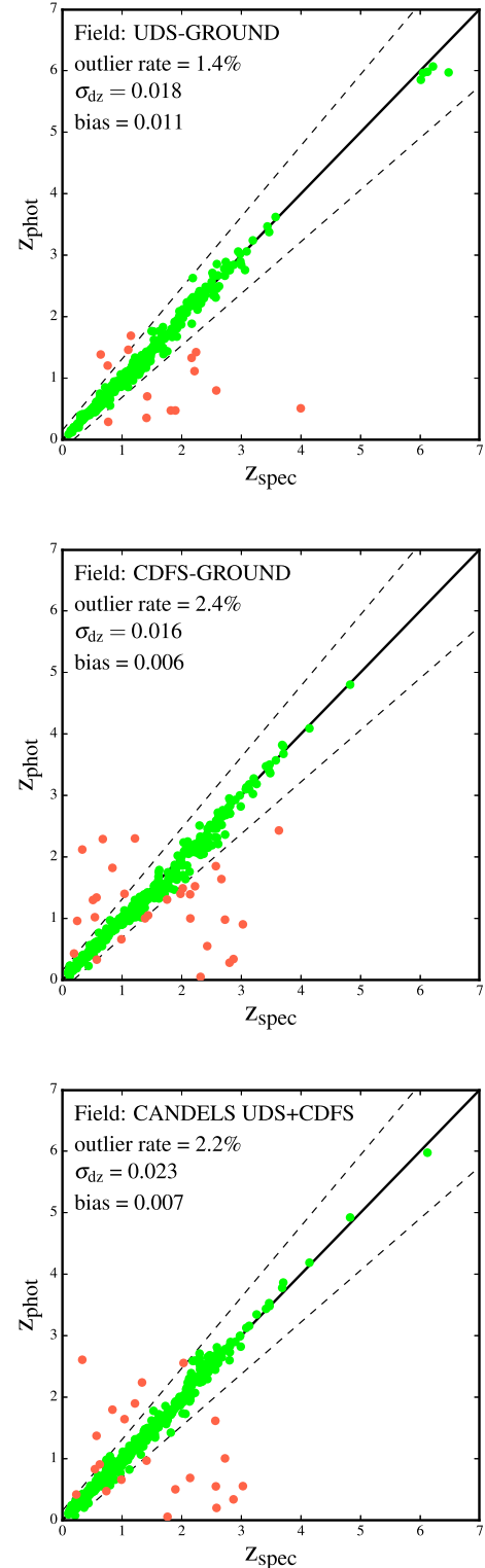
Figure 2. Top: photometric redshifts derived by the VANDELS team compared to robust spectroscopic redshifts in the wide-area region of the UDS (red data points are catastrophic outliers with |dz| > 0.15 ). Middle: equivalent plot for the wide-area region of the CDFS. Bottom: photometric redshift versus spectroscopic redshift for those objects in the top two panels for which photometric redshifts derived by the CANDELS survey team were available (see the text for more details). The catastrophic outlier fraction, \sigma_{dz} and bias are displayed in the top-left corner of each panel.
