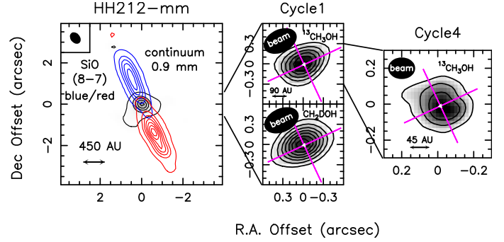
Fig. 1. Left panel: HH212 protostellar system as observed by ALMA-Band 7 (Codella et al. 2014). Blue and red contours plot the blue- and redshifted \text{SiO}(8\text{--}7) jet overlaid on the continuum at 0.9 \text{ mm} (black contours). Positions are with respect to the coordinates reported in Sect. 2. The filled ellipse shows the synthesised beam (HPBW): 0''.61 \times 0''.45 . Central panels: zoom-in of the central region as observed by ALMA-Band 7 Cycle 1: ^{13}\text{CH}_3\text{OH}(13_{0,13}\text{--}12_{1,12})\text{E} and \text{CH}_2\text{DOH}(9_{0,9}\text{--}8_{1,8})\text{e0} integrated over \pm 4 \text{ km s}^{-1} with respect to the v_{\text{sys}} = +1.7 \text{ km s}^{-1} (black contours and grey scale). First contours and steps are 5\sigma for ^{13}\text{CH}_3\text{OH} ( 15 \text{ mJy beam}^{-1} \text{ km s}^{-1} ) and \text{CH}_2\text{DOH} ( 35 \text{ mJy beam}^{-1} \text{ km s}^{-1} ). The HPBWs are 0''.52 \times 0''.34 ( \text{PA} = -64^\circ ) for ^{13}\text{CH}_3\text{OH} and 0''.54 \times 0''.35 ( \text{PA} = -65^\circ ) for \text{CH}_2\text{DOH} . Right panel: zoom-in of the central region, as observed by ALMA-Band 7 Cycle 4, showing the ^{13}\text{CH}_3\text{OH}(12_{1,11}\text{--}12_{0,12})\text{A} emission integrated over 10 \text{ km s}^{-1} around v_{\text{sys}} (black contours and grey scale). First contours and steps are 5\sigma ( 20 \text{ mJy beam}^{-1} \text{ km s}^{-1} ) and 3\sigma , respectively. The HPBW is 0''.15 \times 0''.12 ( \text{PA} = -88^\circ ).
