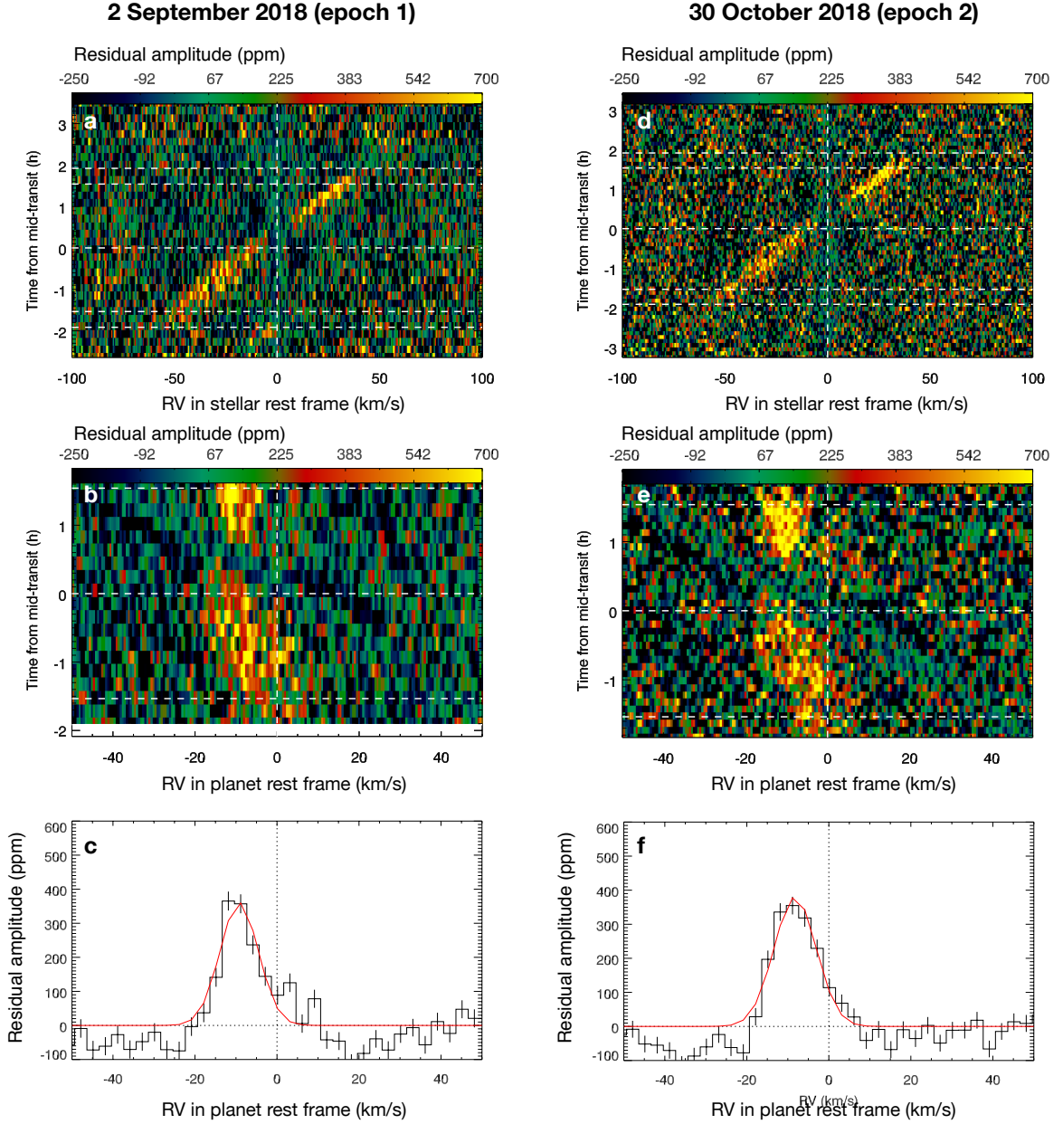
Extended Data Figure 6 | Absorption signature of WASP-76b. a,b,c , On 2 September 2018 (epoch 1). d,e,f , On 30 October 2018 (epoch 2). The planetary absorption signal is shown in the stellar rest frame ( a,d ), the planet rest frame ( b,e ) and is time-averaged in the planet rest frame to produce the atmospheric absorption profile integrated over the whole limb ( c,f ). An indicative Gaussian fit (red curves) is overplotted on the absorption profiles. Both epochs show compatible results.
