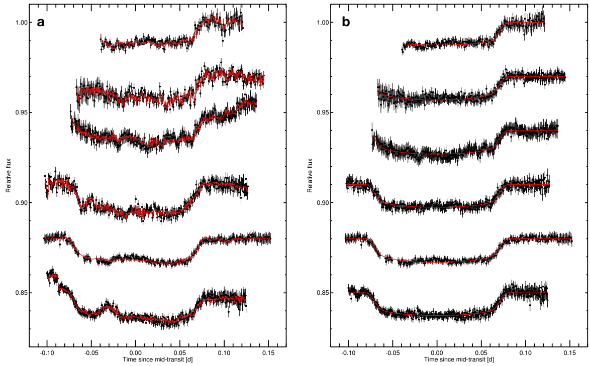
Extended Data Figure 8 | Photometric transit light curve of WASP-76b obtained with the EulerCam instrument on the Swiss Euler 1.2 m telescope in La Silla, Chile. The last three transits (bottom rows) have been previously reported in ref. [19]. a , Raw light curves with their best-fit models including systematic effects. b , Normalised light curves.
