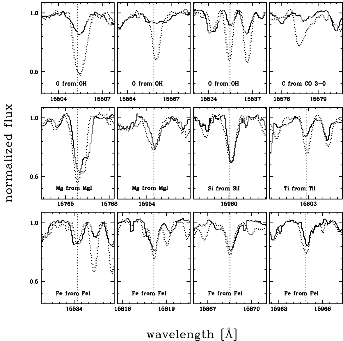
Fig. 2. CRILES spectra centered on some lines of interest of two giant stars (#11, continuous line and #12, dotted line) with very similar abundances but very different temperatures. The coolest giant (#12 at T_{\text{eff}} = 3600 K) has much deeper molecular OH and CO lines than the warmest one (#11 at T_{\text{eff}} = 4250 K).
