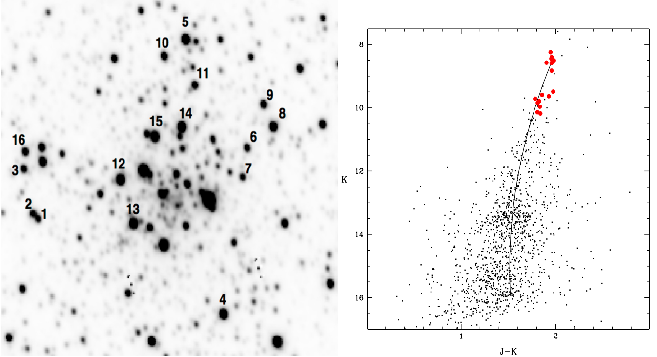
Fig. 1. Left panel: soft K-band image of the core region of Terzan 1. The field of view shown in the map is \sim 1' \times 1' , north is up and east on the left. The observed stars are numbered (cf. Table 1). Right panel: observed K, (J-K) CMD, and mean RGB ridgeline of Terzan 1 in the central \sim 1 arcmin in radius from Valenti et al. (2010). Large red filled points denote the stars observed spectroscopically.
