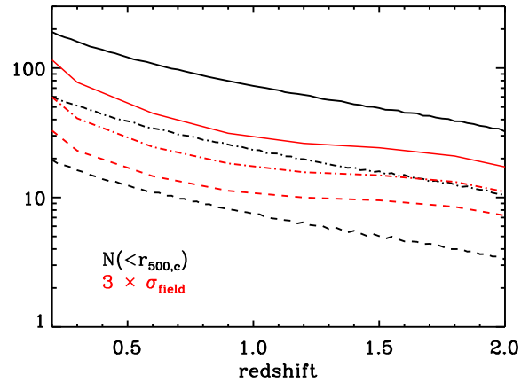
Figure 1. Number N_{500,c} of cluster galaxies within r_{500,c} (black curves), and 3\sigma_{\text{field}} , where \sigma_{\text{field}} is the rms of the field counts within the same radius, and within the adopted 3\Delta z_p cut (red curves). These counts are shown down to the limiting magnitude of the Euclid survey, H_{AB} = 24 , as a function of redshift for clusters of different masses, \log(M_{200,c}/M_\odot) = 14.5, 14.0, 13.5 (solid, dot-dashed, dashed line, respectively), where masses are defined with a mean overdensity of 200 times the critical density of the Universe at the cluster redshifts.
