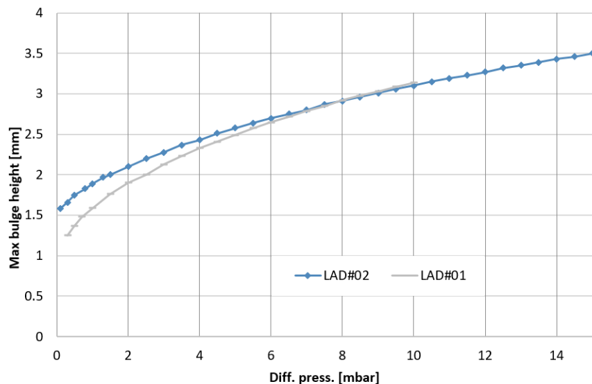
Figure 11. Measures of the maximum bulge height vs. differential pressure applied to the filters.
