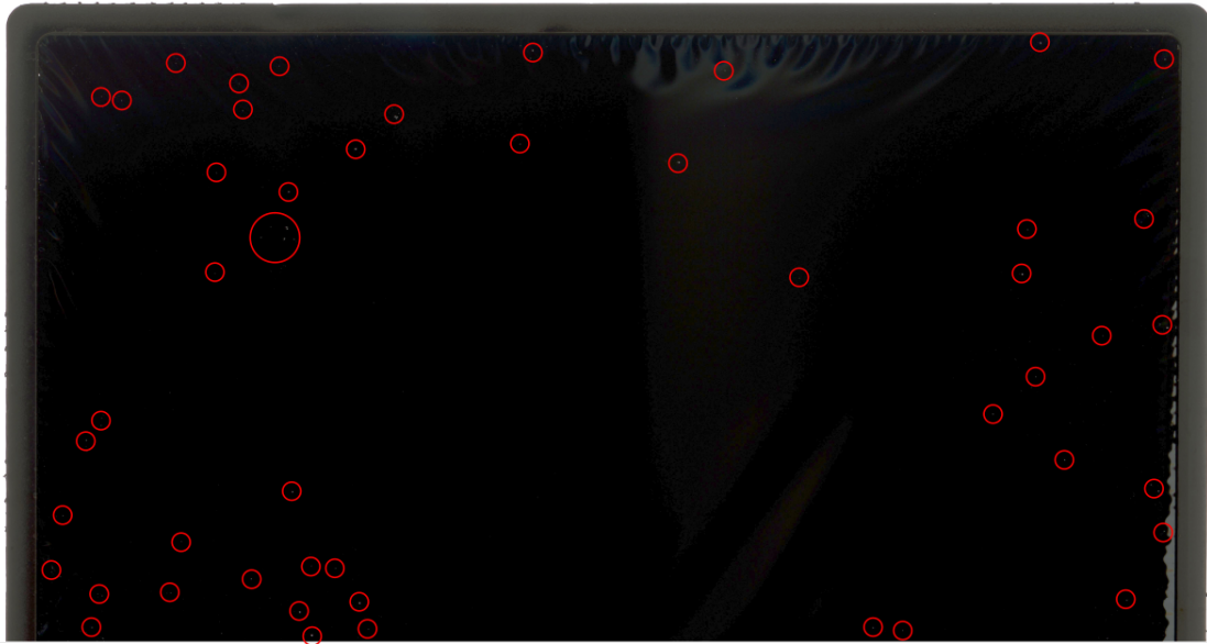
Figure 8. Portion of a filter prototype image acquired in transmission mode with a high resolution scanner. The membrane is 2\ \mu\text{m} of PI and 200 nm of aluminum. Early prototypes such as this presented a high number of pinholes, highlighted in the picture by red circles.
