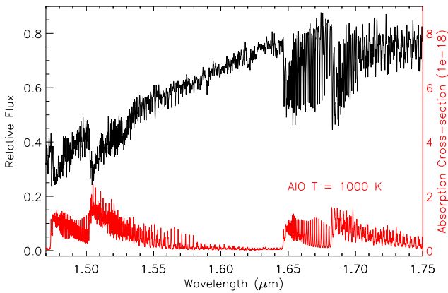
Figure 4. The H -bandpass spectrum of L222.59 with an analytical model of the AIO absorption bands from ExoMol (red lines; Bowesman et al. 2021).
