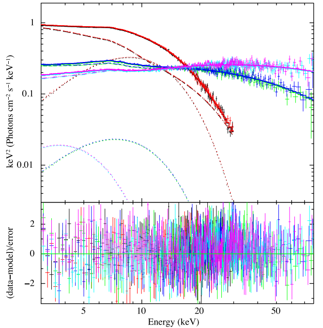
Figure 7. NuSTAR unfolded spectra and models fitted with the model \text{CONST*PHABS*(BBODY+RELXILL)} for 4U 1636–53. Colours are the same in Fig. 2. The dot and dash-dotted line represent the BBODY and RELXILL components in this model. The bottom panel shows the residuals in terms of sigmas. The corresponding parameters are given in Table 4.
