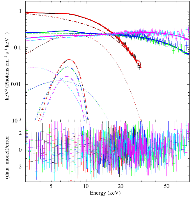
Figure 3. NuSTAR unfolded spectra and models fitted with the model CONST*PHABS*(BBODY+GAUSSIAN+NTHCOMP) for 4U 1636–53. The colours are the same as in Fig. 2. The dot, dash and dash-dotted lines represent the BBODY, GAUSSIAN and NTHCOMP components in our model, respectively. Notice that in the top panel of the following spectra figures, the y-axis always shows E^2 f(E) . The bottom panel shows the residuals in terms of sigmas. The best-fitting parameters are given in Table 2.
