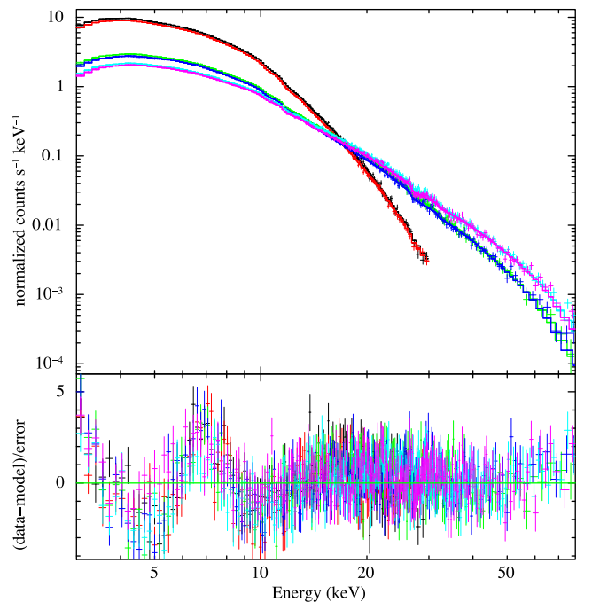
Figure 2. NuSTAR spectra and models for the fit with CONST*PHABS*(BBODY+NTHCOMP) for 4U 1636–53. The black, red, green, blue, light blue and magenta lines in the top panel represent each spectrum (FPMA/B) listed from top to bottom in Table 1, separately. The bottom panel shows the residuals in terms of sigmas; the colours are the same as in the top panel. The spectra have been rebinned for plotting purposes.
