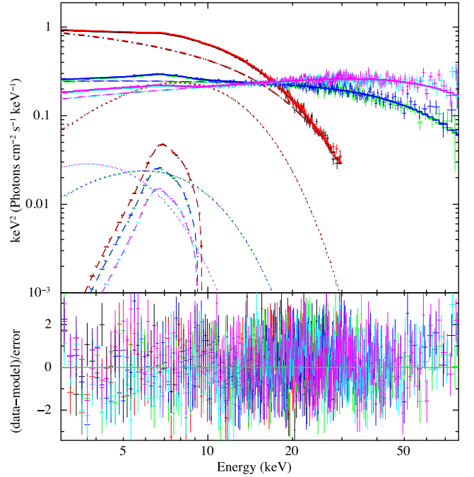
Figure 4. NuSTAR unfolded spectra and models fitted with the model CONST*PHABS*(BBODY+KYRLINE+NTHCOMP) for 4U 1636–53. Colours and lines are the same as in Fig. 2, except for the dash-dotted line representing the KYRLINE component in this model. The bottom panel shows the residuals in terms of sigmas. The corresponding parameters are given in Table 3.
