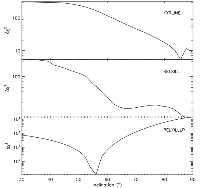
Figure 5. The change in the goodness of fit, \Delta\chi^2 , versus the inclination of different models for the NuSTAR observations of 4U 1636–53. The \Delta\chi^2 was calculated using the command steppar in XSPEC over 30 steps in the inclination angle. The y-axis is in logarithmic scale. The panels from top to bottom correspond to the best fitting of Models 1 to 3, respectively.
