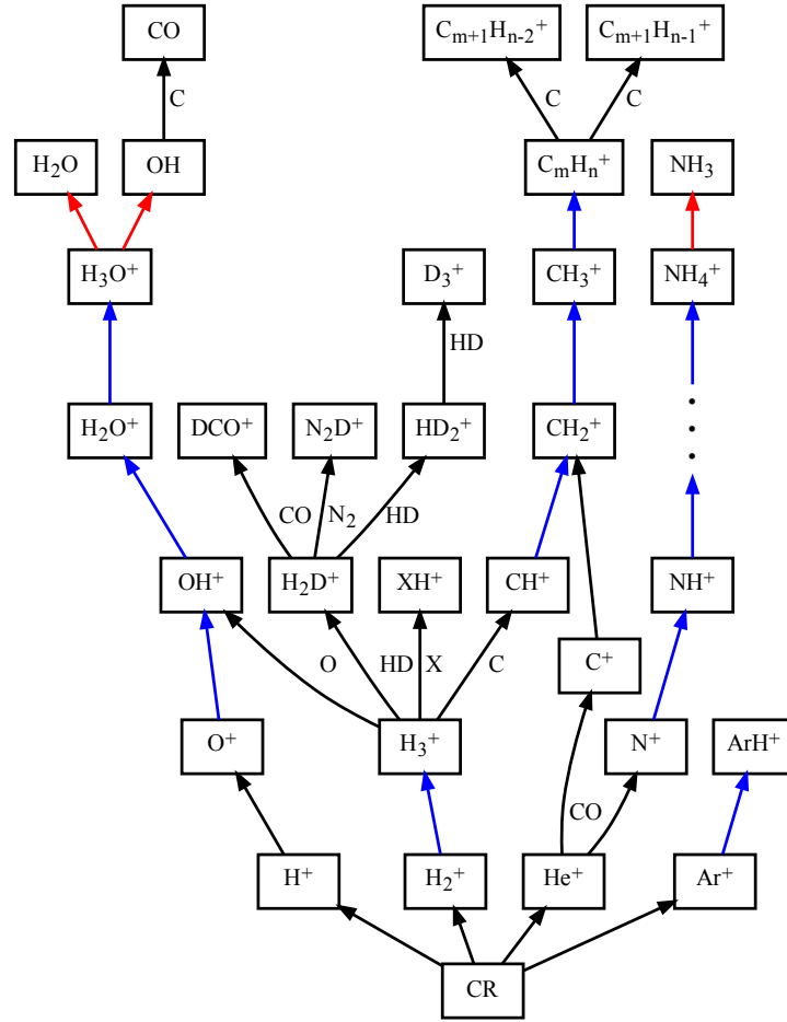
FIGURE 8.3 The cosmic-ray chemistry tree . Blue lines indicate \text{H}_2 interactions, and red lines \text{e}^- recombination. \text{XH}^+ refers to ions produced through the proton transfer reaction, such as \text{N}_2\text{H}^+ and \text{HCO}^+ from \text{N}_2 and \text{CO} , respectively (represented by X). The dots after \text{NH}^+ represent hydrogen abstraction reactions with \text{H}_2 (e.g., \text{NH}^+ + \text{H}_2 \rightarrow \text{NH}_2^+ + \text{H} ).
