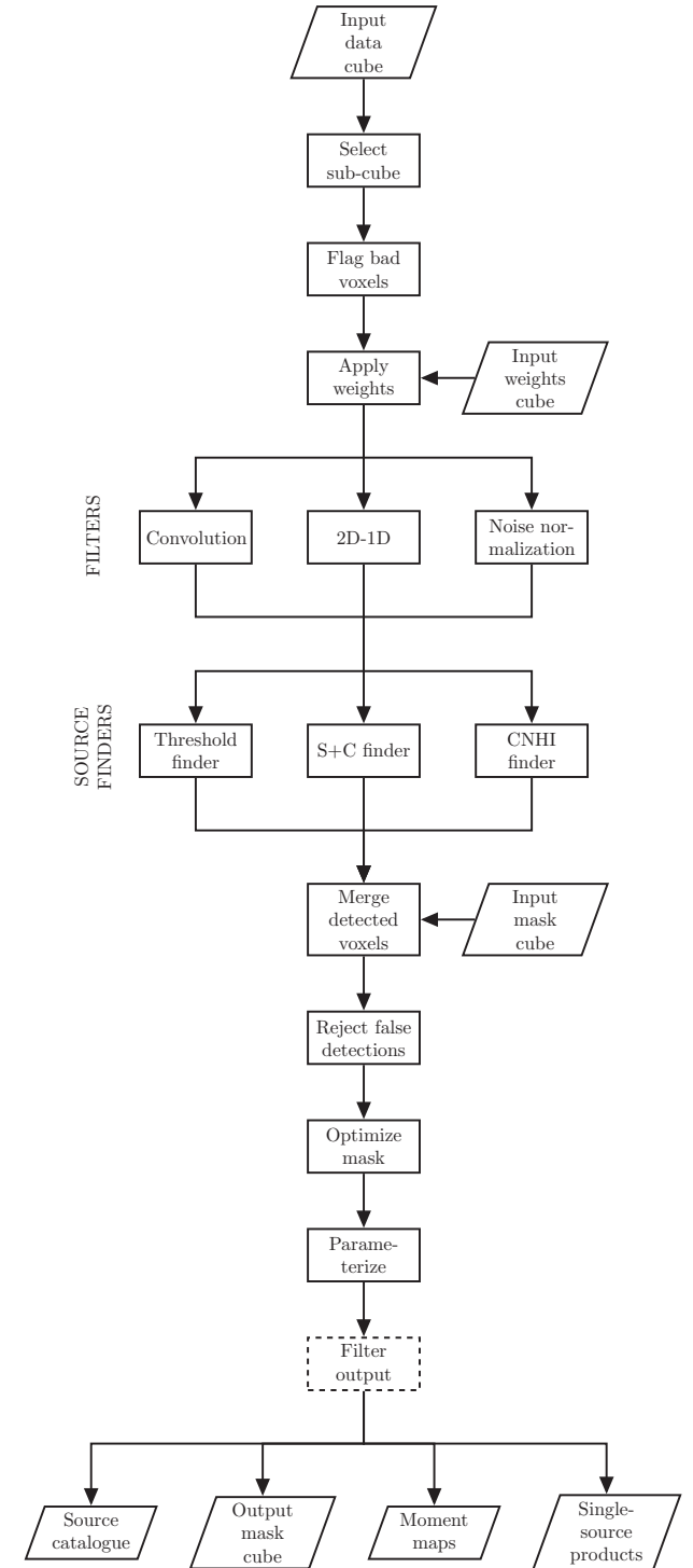
Figure 2. SoFiA flowchart. We highlight the ‘Filter output’ module with a dashed box as this will become available in future releases of SoFiA.
