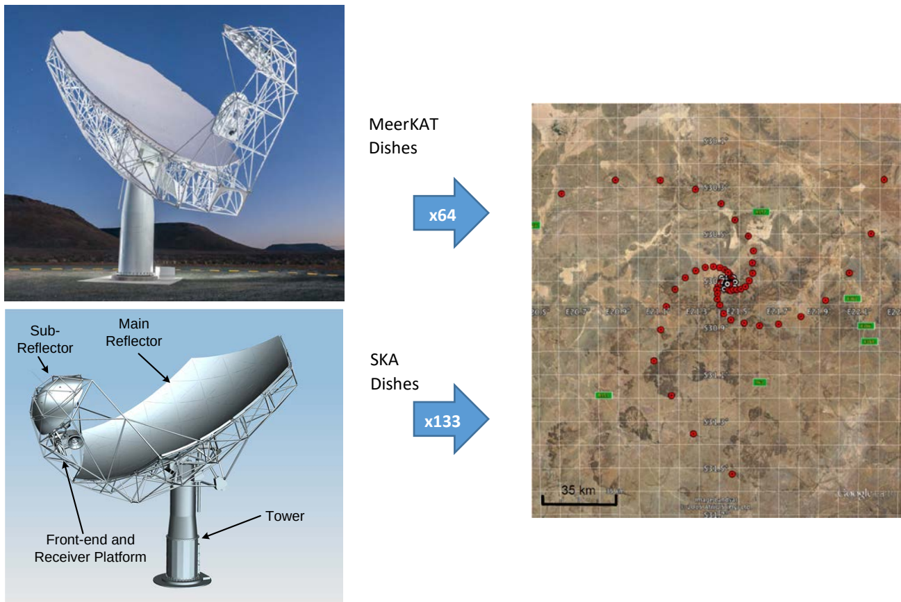
Figure 13. SKA1-MID integrates the 64 existing MeerKAT (top left) dishes with 133 new SKA-1 dishes (bottom left).
