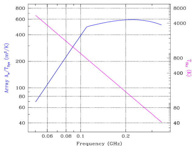
Figure 8: Sensitivity of SKA1-LOW Telescope. Note that the complete requirement (and the T_{\text{sys}} actually assumed) are described more accurately in SKA1-SYS_REQ-2135 and Sect. 26.2 of the SKA1 System Requirements Specification [5]).
