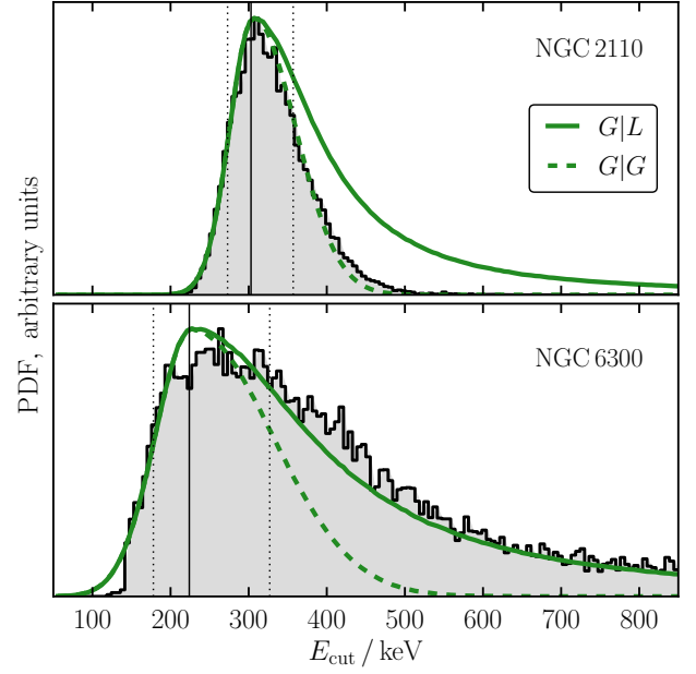
Figure 5. Two illustrative examples of probability density functions (PDFs) derived from MCMC chains for two targets (NGC 2110 in the top panel, and NGC 6300 in the bottom panel), shown as gray histograms, compared to assumed analytic PDFs shown with green curves. Solid lines show the adopted fiducial PDFs composed of a Gaussian and a Lorentzian ( G|L ), while the dashed lines show a two-sided Gaussian ( G|G ). In both cases, the transition occurs at the best-fit value ( E_{\text{cut}}^{\text{b.f.}} ; vertical solid line) and the standard deviation on either side is determined by the extent of the 68 % confidence interval ( E_{\text{cut}}^{\text{l.l.}} and E_{\text{cut}}^{\text{u.l.}} ; vertical dotted lines).
