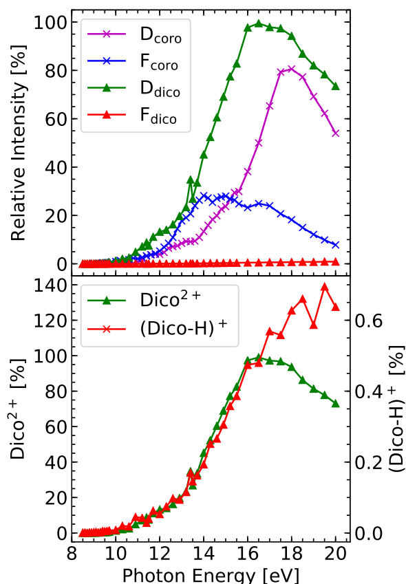
Figure 7. Upper panel: Dication, D, and fragment, F, photoproducts upon VUV photon absorption of coronene, \text{C}_{24}\text{H}_{12}^+ (coro) and dicoronylene, \text{C}_{48}\text{H}_{20}^+ (dico). Lower panel: Comparison of the dication and the H loss channel of dicoronylene.
