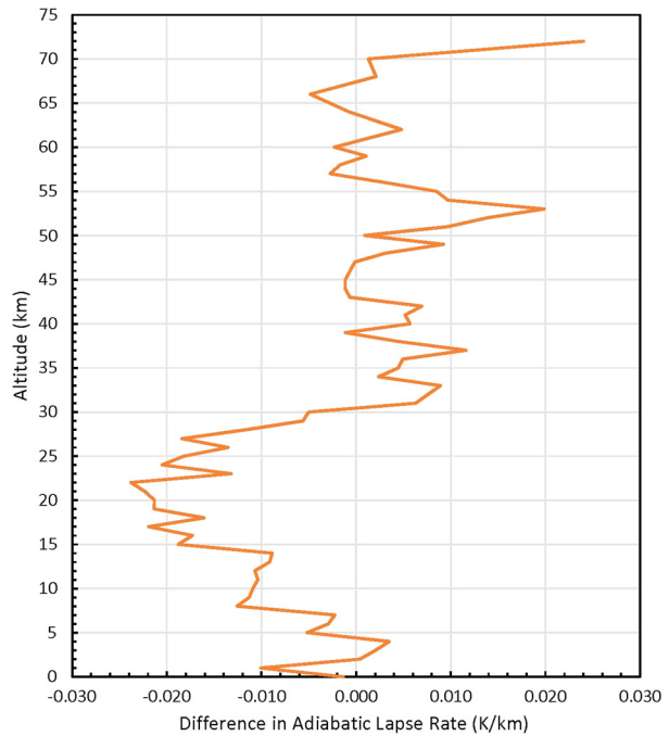
Fig. 23 Differences in the dry adiabatic lapse rates computed for VIRA profile using different real gas equations of state (GERG 2008) and VIRA Model approximation for a 96.5% \text{CO}_2 + 3.5% \text{N}_2 mixture (Dutt and Limaye 2018) and compared with pure \text{CO}_2
