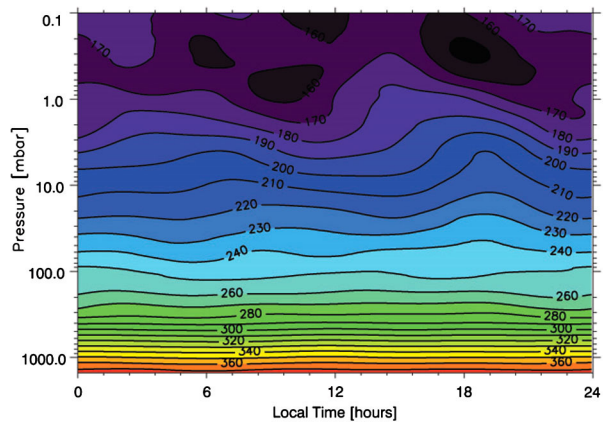
Fig. 21 Thermal structure as a function of local time and pressure in the equatorial region ( \text{lat} \leq \pm 20^\circ ). The thermal structure is approximated by a diurnal mean temperature and the first two tidal modes. A pronounced semidiurnal structure develops in the upper mesosphere around the morning and evening terminators
