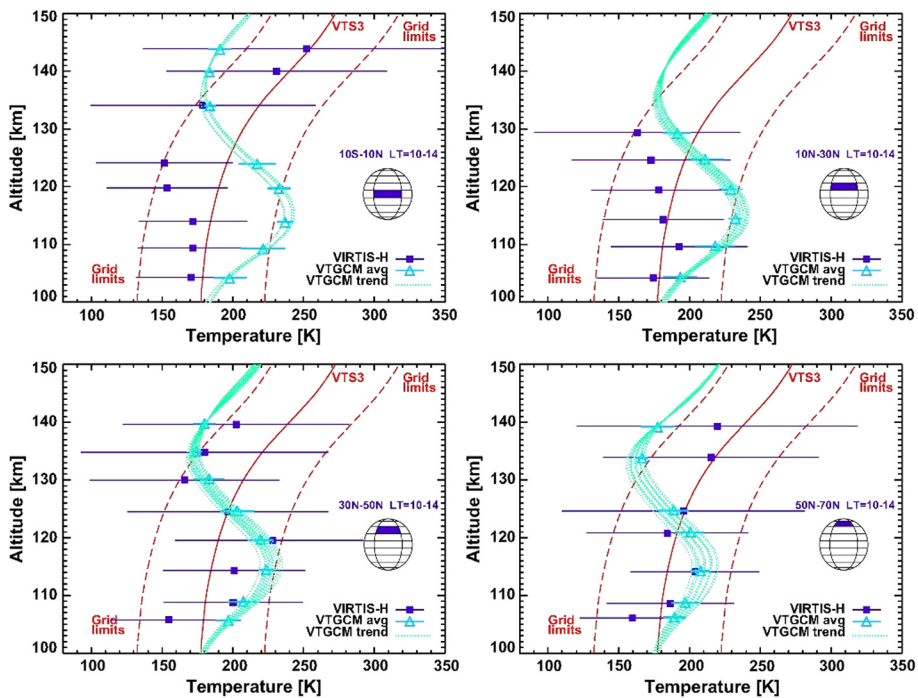
Fig. 9 Retrievals of kinetic temperature and error bars, at local time 10–14 h, as a function of altitude, from VIRTIS-H limb averages. Results at four latitudes are shown in the four panels, as indicated in the legends: 10° S–10° N (top-left panel), 10° N–30° N (top-right), 30° N–50° N (bottom-left) and 50° N–70° N (bottom-right). VTGCM (Bougher et al. 2015) daytime average temperature, corresponding to the VIRTIS-H selected boxes, are shown with their error bars (purple squares and lines). A set of profiles from the VTGCM are also shown with dotted-green lines, labeled as “VTGCM trend”, which are individual outputs of the VTGCM within the VIRTIS latitude-local time bins. The VTS3 profile (solid red line), and the grid limits (dashed red lines) are shown for reference. (From Gilli et al. 2015)
