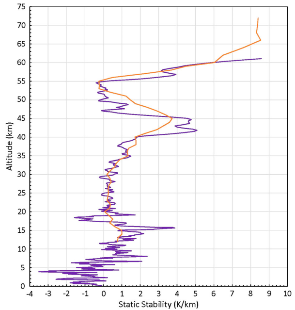
Fig. 24 Static stability of the VeGa 2 lander temperature profile calculated using the adiabatic lapse rate from the real gas equation of state (Dutt and Limaye 2018) for \text{CO}_2 + \text{N}_2 mixture confirms the unstable layer below 7 km (shown in purple). The VIRA deep atmosphere adiabatic lapse rate (Tables 1.1 and 1.2 from Seiff et al. 1985) is also shown (orange)
