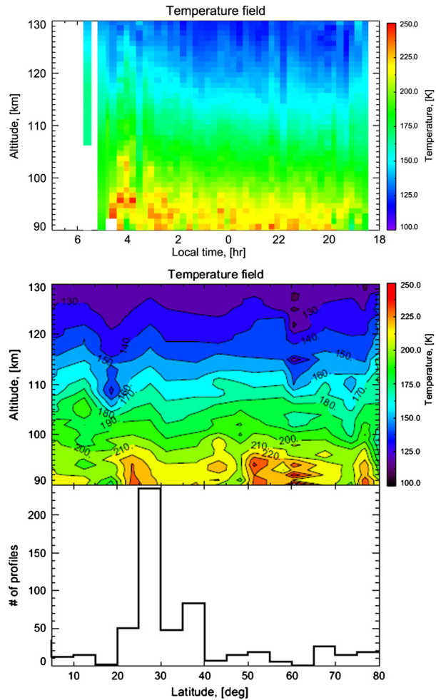
Fig. 22 (Top) Temperature variation with local time and altitude and with latitude and altitude cross section from SPICAV temperature profiles. The latitudinal sampling from the SPICAV occultations is not uniform as can be seen in the sampling shown in the bottom panel. 587 profiles are used in generating these cross sections. (From Piccialli et al. 2015)
