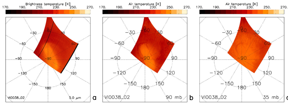
Fig. 2 Analysis of VIRTIS-M cube V10038_02. Panels a–c present the radiance measured at 5 \mu\text{m} and the temperatures retrieved at the levels of 90 mb and 35 mb respectively. (From Grassi et al. 2008.) The vertical dependence of the night time temperatures is shown in Fig. 6
