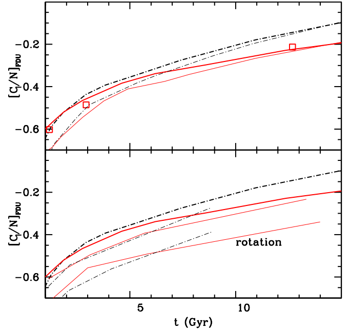
Fig. 3. Comparison between the BaSTI (thick lines, upper panel), STAREVOL (thin lines, lower panel) predictions for the [\text{C}/\text{N}]_{\text{FDU}} - t relation at selected metallicities. BaSTI results for [\text{M}/\text{H}] = 0.06 (solid line) and [\text{M}/\text{H}] = -0.66 (dash-dotted line) are displayed together with PARSEC results for [\text{M}/\text{H}] = -0.02 (solid line) and [\text{M}/\text{H}] = -0.58 (dash-dotted line), and STAREVOL results for [\text{M}/\text{H}] = 0.0 (solid line) and [\text{M}/\text{H}] = -0.56 (dash-dotted line). STAREVOL models with rotation for the same metallicities are also displayed (with the same line styles). In the upper panel squares denote BaSTI calculations for [\text{M}/\text{H}] = 0.04 and the Caffau et al. (2011) solar heavy element distribution (see text for details).
