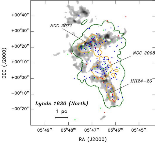
Fig. 8. Distribution of young stellar objects plotted over the extinction map (in gray) of the region. The green and orange contours correspond to volume densities of 1 M_{\odot} pc^{-3} and 10 M_{\odot} pc^{-3} , respectively. Class I sources are shown in red, flat spectrum sources in green, and Class II sources in blue.
