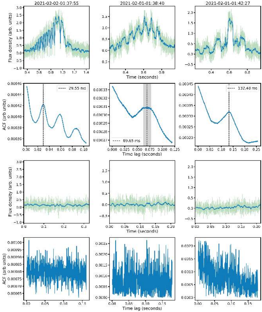
Extended Data Figure 2: Examples of quasi-periodic pulses. The top two rows show pulse profiles and their corresponding ACFs at 306.24\mu\text{s} resolution, respectively. The value the of quasi-period is indicated by the black vertical lines. The bottom two rows show the off-pulse regions and their corresponding ACFs.
