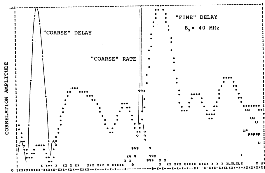
Fig. 3 Multichannel delay resolution function (Mk III fringe analysis)
