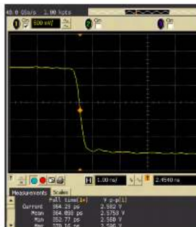
Fig 1b: Example fall time of 364 ps
