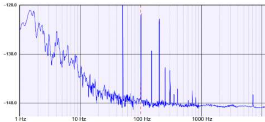
Fig 4b: Phase noise of 10 MHz square wave output, input 10 MHz sine, 13 dBm to input B, trigger 0V
