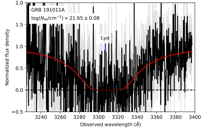
Fig. A.7. Same as Fig. A.1 but for GRB 191011A, with a best-fit \log(N_{\text{HI}}/\text{cm}^{-2}) = 21.49 \pm 0.03 .
