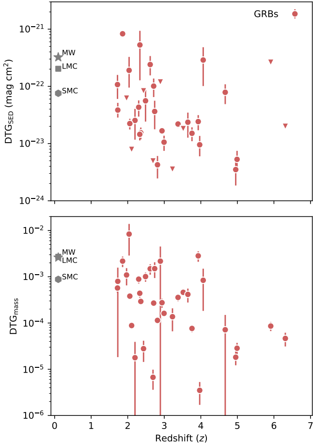
Fig. 6. SED-derived DTG ratio, \text{DTG}_{\text{SED}} = A_V/N_{\text{HI}} (top), and depletion-derived \text{DTG}_{\text{mass}} (bottom) as a function of redshift. The symbol notation follows Fig. 3. For comparison we mark the DTG ratios of the MW, LMC, and SMC. The GRB sightlines through high-redshift galaxies typically probe lower DTG content than inferred from these local galaxies.
