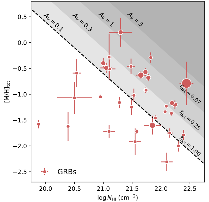
Fig. 8. Dust-corrected metallicity as a function of H I column density. The red dots again represent the main GRB sample but here are size-coded as a function of the SED-derived A_V . The gray-shaded regions represent increasing A_V , marked for each region, assuming the constant \text{DTM}_{\text{SED}} ratio derived in this work of \log A_V - [\log N_{\text{HI}} + [\text{M}/\text{H}]_{\text{tot}}] = -21.4 . The estimated detection probability for GRBs in each of these A_V ranges is marked as well (see Sect. 4.4 for further details).
