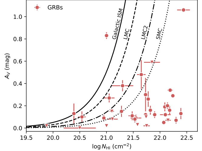
Fig. 5. Visual extinction ( A_V ) vs. \text{H I} column density ( N_{\text{HI}} ), i.e., the DTG ratio. The symbol notation follows Fig. 3. For comparison are overplotted the average DTG ratios from specific sightlines in the Local Group (MW, LMC, LMC2, and SMC) from Gordon et al. (2003). GRBs typically probe sightlines with lower A_V for a given N_{\text{HI}} than the local galaxies.
