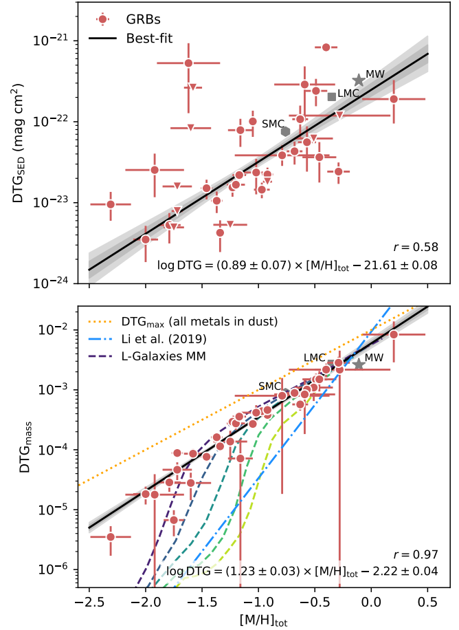
Fig. 7. SED-derived DTG ratio, \text{DTG}_{\text{SED}} = A_V/N_{\text{HI}} (top), and depletion-derived \text{DTG}_{\text{mass}} (bottom) as a function of dust-corrected metallicity, [\text{M}/\text{H}]_{\text{tot}} . The symbol notation follows Fig. 3. We find strong correlations between the DTG inferred both from the SED (top panel) and from depletion (bottom panel) with the metallicity. In the bottom panel we also show the predictions from the Simba simulation at z \sim 0 – 6 (dotted blue line; Li et al. 2019) and the L-Galaxies MM simulation at z \sim 2 – 6 (dashed lines; Yates et al., in prep.). The dashed orange line is the limit at which all metals are incorporated into grains (DTM = 1).
