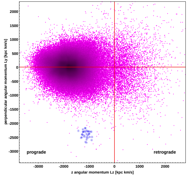
Fig. 25. Distribution of DR2 stars in a circle of 15 degrees radius around the Galactic anticentre direction in the L_\perp = L_y vs L_z space. The Helmi stream is the distinct density enhancement near the bottom of the plot (in blue). We have assumed here v_{rot} = 220 km s -1 for the LSR velocity, v_{z,\odot} = 5 km s -1 , and v_{\phi,\odot} = 7 km s -1 for the peculiar motion of the Sun, and R_\odot = 8.1 kpc.
