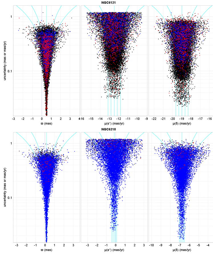
Fig. A.4. Two examples of the parallax and PM dispersion diagrams for clusters at a distance of approximately 2 (top) and 5 (bottom) kpc. The parallax and PMs are plotted against the standard uncertainties. The blue lines show the expected uncertainty levels relative to the mean value at -2 , -1 , 0 , 1 and 2 \sigma , including noise contributions from the internal velocity dispersion and the dispersion of the parallaxes from the depth of the cluster. At low levels of standard uncertainty, the contributions from the internal dispersion are easily detected. The colouring of the data points reflects the error correlations: red means strongly negative, blue means strongly positive, and black means low.
