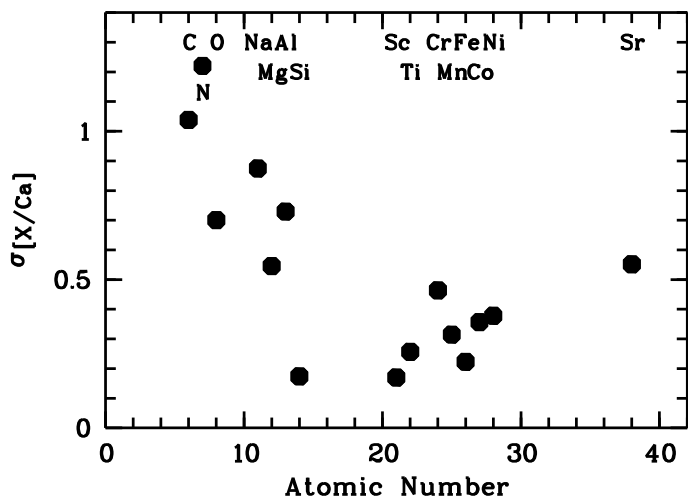
Fig. 8. The \sigma [X/Ca] for elements that are measured in at least two of the nine CEMP stars (HE 0107-5240 HE 1327-2326, HE 0557-4840, HE 0134-1519, HE 0233-0343, HE 1310-0536, SMSS J0313-6708, CS 22949-037, and G 77-61), as a function of atomic number. As in Fig. 7, C and N in CS 22949-037 were not taken into account.
