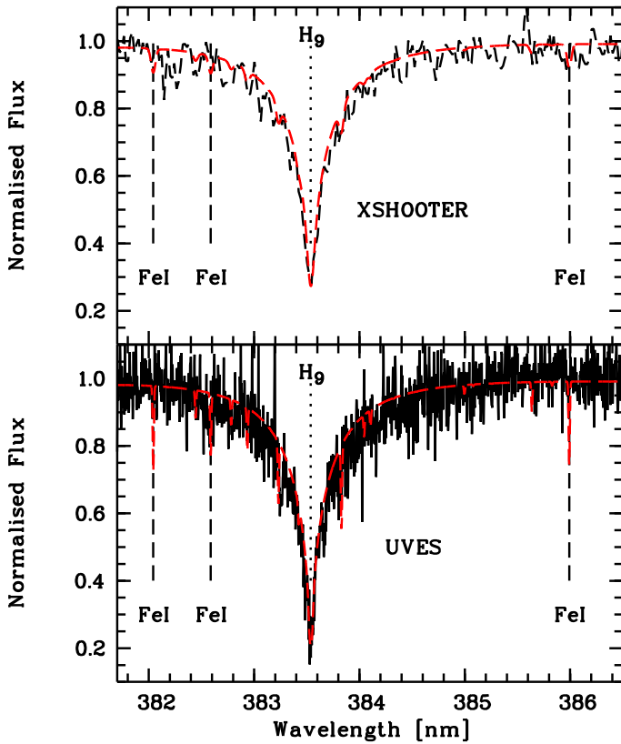
Fig. 4. SDSS J1035+06411: the X-Shooter (top panel) and UVES (bottom panel) spectra in the region covering the three strongest Fe I lines. The comparison spectrum is a synthetic spectrum computed with [\text{Fe}/\text{H}] = -4.5 .
