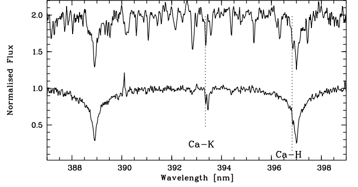
Fig. 2. The X-Shooter spectra around the Ca II H & K lines of SDSS J0929+0238 (the spectrum is vertically displaced by 1 unit for display purposes) and SDSS J1035+0641. The dotted lines mark the position of the stellar Ca II H & K lines. The CH lines are much more prominent in the former because the carbon abundance is almost 1 dex larger and the effective temperature is almost 300 K cooler.
