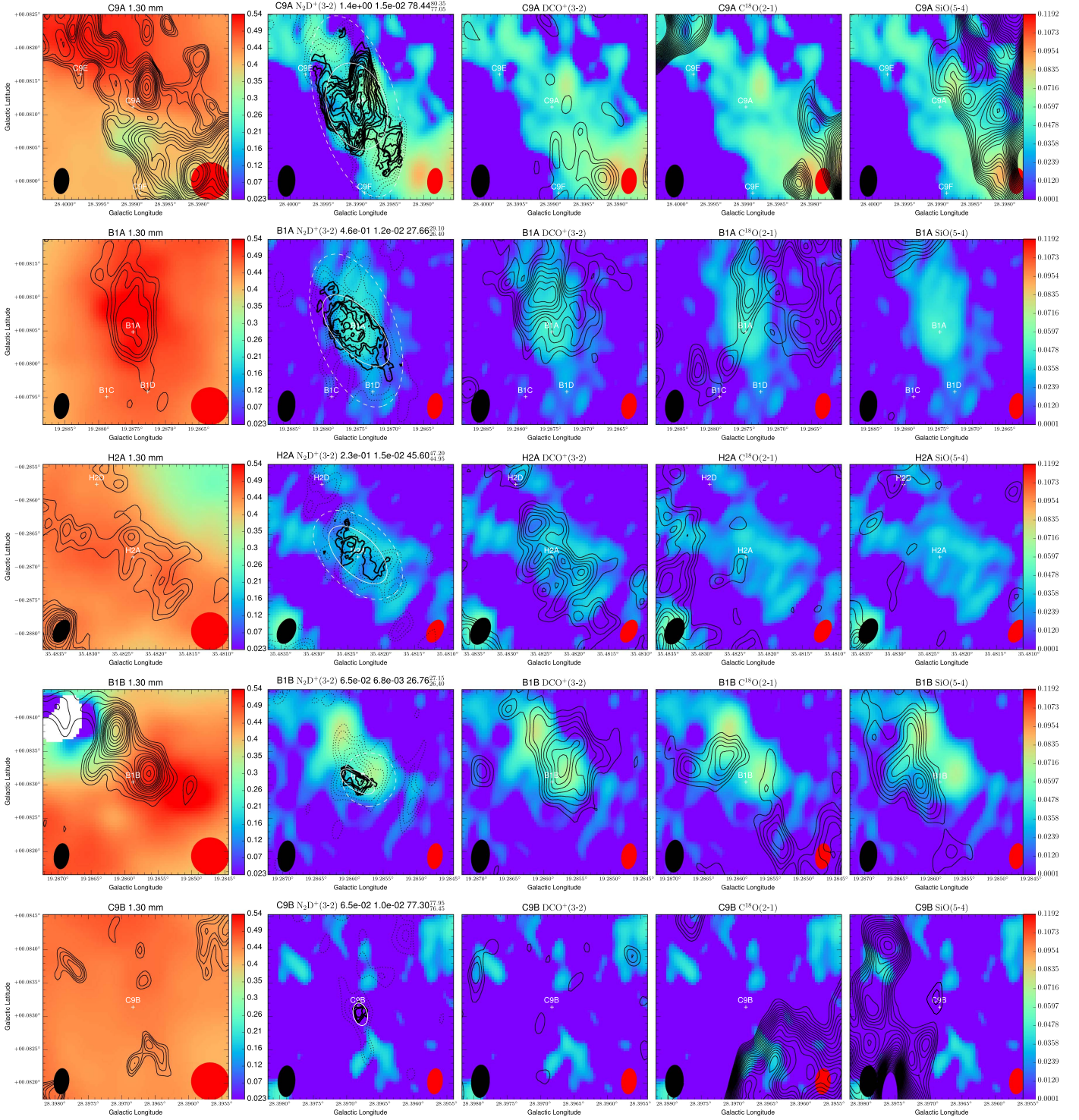
Figure 11. Core-scale zoom-in figures of C9A, B1A, H2A, B1B, C9B (rows top to bottom, also following rank order of \text{N}_2\text{D}^+(3-2) flux). Each panel shows a 10'' by 10'' FOV. The first column shows 1.3\text{ mm} continuum (contours: 2, 3, 4, 5, 7, 9, 11, 13, 15, 17, 20, 40, 60, 80... \sigma , where 1\sigma \simeq 2.2 \times 10^{-4} \text{ Jy beam}^{-1} ; ALMA beam in lower left) overlaid on MIREX (BT12) mass surface density (color scale in \text{g cm}^{-2} ; Spitzer beam in lower right). 2nd column shows 0th-moment \text{N}_2\text{D}^+(3-2) of the cores (only including core voxels), shown as the solid contours: 2, 3, 4, 5... \sigma (beam lower left), overlaid on the 1.30\text{ mm} continuum (beam lower right). The dotted contours are the full integration of the cores (including all voxels within the channels). At the top of the panel we list total \text{N}_2\text{D}^+(3-2) flux (in \text{Jy beam}^{-1} \text{ km s}^{-1} ), \text{N}_2\text{D}^+(3-2) 0th-moment map rms (in \text{Jy beam}^{-1} \text{ km s}^{-1} ), and \text{N}_2\text{D}^+(3-2) intensity weighted core velocity and velocity range (in \text{km s}^{-1} ). The solid and dashed ellipses are fitted boundaries to the cores (see text). 3rd column is the same as the 2nd, except contours now show \text{DCO}^+(3-2) integrated over the same velocity range as the \text{N}_2\text{D}^+ core. 4th column is the same as the 2nd, except contours now show \text{C}^{18}\text{O}(2-1) integrated over the same velocity range as the \text{N}_2\text{D}^+ core. 5th column is the same as the 2nd, except contours now show \text{SiO}(5-4) integrated over the 5 \text{ km s}^{-1} velocity range used in the region maps.
