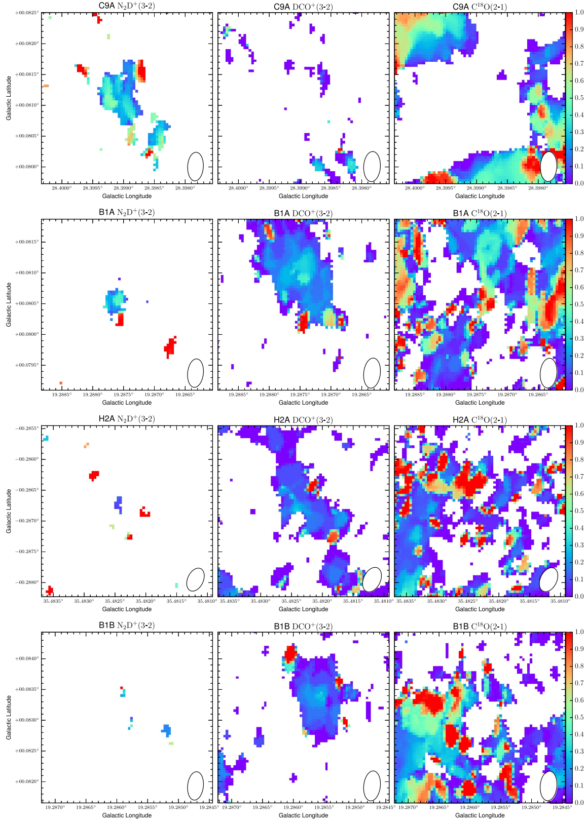
Figure 15. Second-moment (intensity-weighted velocity dispersion) maps of the top four ranked N 2 D + (3-2) cores C9A (first row), B1A (second row), H2A (third row), B1B (fourth row), in N 2 D + (first column), DCO + (second column), C 18 O (third column). The calculation is within a 5 km s -1 range, centered on N 2 D + v_{\text{LSR}} (Table 2). Only voxels with \geq 3\sigma intensity are considered and shown in color. For the N 2 D + data, a 0.242 km s -1 contribution to the dispersion from the main group of hyperfine structures is subtracted in quadrature. However, we see in some regions the second-moment pixels shrink from the first-moment images. This is mainly due to the fact that the velocity span is narrower than 0.242 km s -1 . In these areas, we are limited by the sensitivity. The color scale is linear from 0 to 1.0 km s -1 . The synthesized beam is shown in the lower-right corner.
